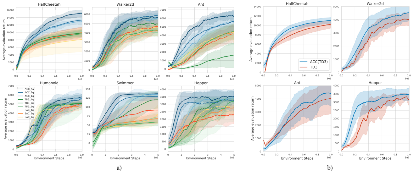
Fig. 3. The mean \pm standard deviation over 10 trials, which is the common metric for non-aggregated results since the bootstrapped confidence intervals are less reliable for 10 trials (cf. A.3 in [23]). (a) Results in the sample efficient regime where tuning of hyperparameters in an inner loop is too costly with different choices for the number of value function updates per environment step. (b) Results for ACC applied to TD3 compared to pure TD3.
