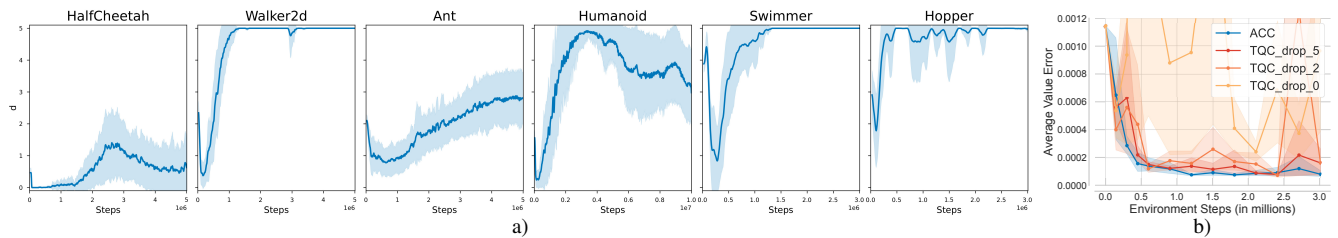
Fig. 4. (a) Mean (thick line) and standard deviation (shaded area) over 10 trials of the number of dropped targets per network d = d_{max} - \beta in ACC over time for different environments with a uniform filter of size 15. (b) The normalized absolute error of the value estimate aggregated over the 6 environments. Shown are the mean with stratified bootstrapped confidence intervals computed from the results of 5 trials per environment. We used a uniform filter of size 401 for readability.
