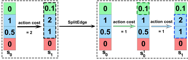
Figure 5: Example of the SPLITEDGE process ensuring minimal action cost. The edge between states s_0 and s_1 (left box) has an action cost of 2 changing the green and blue factors. Each color represents a factored state space with values corresponding to object joint values. Applying SPLITEDGE creates two edges, which changes first the green factor space, then the blue factor space. This results in two states, s'_0 and s_1 .
