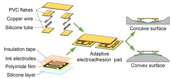
Fig. 2. Structure of adaptive EA pad. The adaptive EA pad can adapt to concave and convex surfaces due to two rotatable EA pads.
