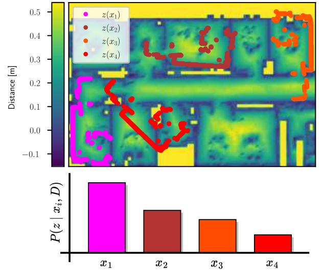
Fig. 4: The neural distance field can be used in a particle filter to evaluate the likelihood of a measurement for each particle in the given NDF. The better the scans are aligned with the zero level of the NDF, the higher the likelihood.
