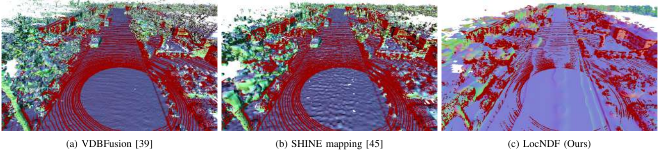
Fig. 5: Qualitative results of registering a scan (red points) to the maps generated by different distance field-based methods. The meshes are generated using the marching cubes algorithm. We use the mesh only for visualization purposes, the registration is done directly on the distance field.
