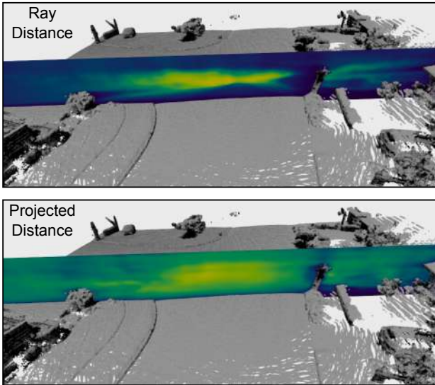
Fig. 7: A visualization of the distance fields when supervising the distance field with the ray distance (top), as well as with the projected distance (bottom). The distance fields are evaluated on a slice in the middle of the scene and depicted by the color. When using the ray distance, one can see the field of view of the LiDAR sensor, leading to a gradient from the surface to the LiDAR center. For the projected distance on the other hand it looks more like a true Euclidean distance field where the gradient ascends radially from the surface. Note, that the NDF is only supervised for the regions within the field of view of the sensor, leading to wrong values in unobserved areas.
