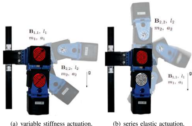
Fig. 1. Examples of articulated soft robots with joints that present torsional springs. The red joints are actuated, while the white one is unactuated. (a) Two degrees of freedom robot actuated by VSA performing a regulation task. (b) Two degrees of freedom robot with an actuated SEA joint, and an unactuated elastic joint.
