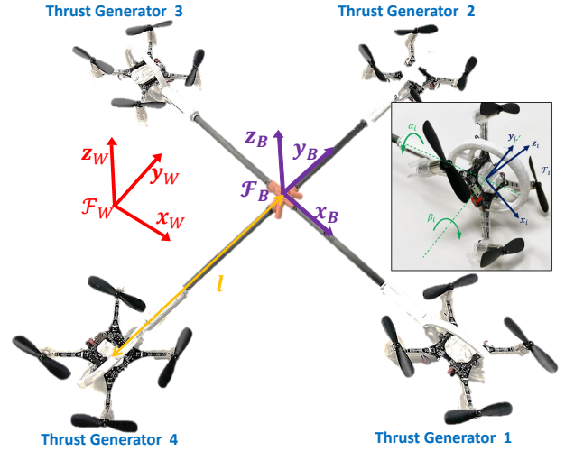
Fig. 2: The coordination system of the over-actuated UAV platform. Four normal quadcopters are mounted on the 2-DoF gimbal mechanisms to provide omni-directional thrust generation capability.
