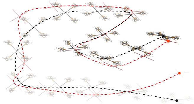
Fig. 1: Utilizing the proposed dynamic-consistent motion planner, the over-actuated UAV platform successfully tracks a dynamic target in real-time. The trajectories of the target and over-actuated UAV are plotted in red and black dash lines, respectively. Corresponding initial and final configurations are plotted as dots and stars, respectively.
