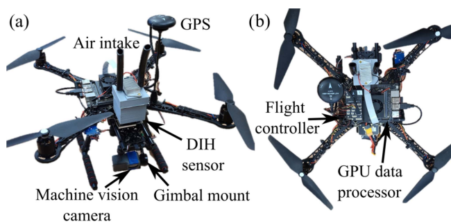
Fig. 2. UAV hardware including all on-board sensors, with a front view shown in (a) and a top-down view shown in (b).
