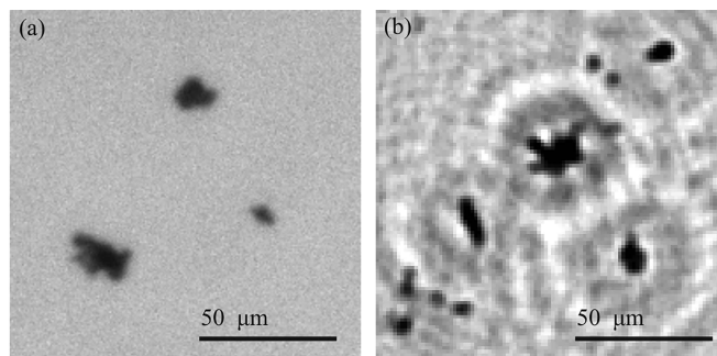
Fig. 6. Soot particles collected from smoke grenade residue imaged with (a) traditional brightfield microscope with 0.75 \mu\text{m}/\text{pix.} resolution, and (b) similar particles from the same residue captured and imaged by the DIH sensor.
