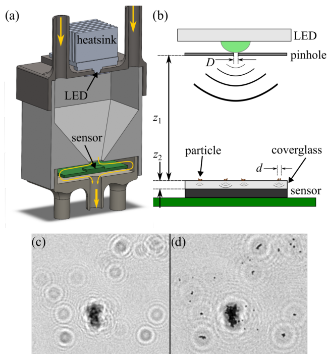
Fig. 5. Sensor for particle diagnostics using digital inline holography. (a) Shows the internal structure of the enclosure, with airflow direction indicated with yellow arrows, where air is pumped in from the top. (b) Depicts the optics of the lensless holographic imaging (not to scale). (c)–(d) Shows hologram examples obtained from the sensor in (a)–(b) before and after focusing the image with holographic reconstruction.
