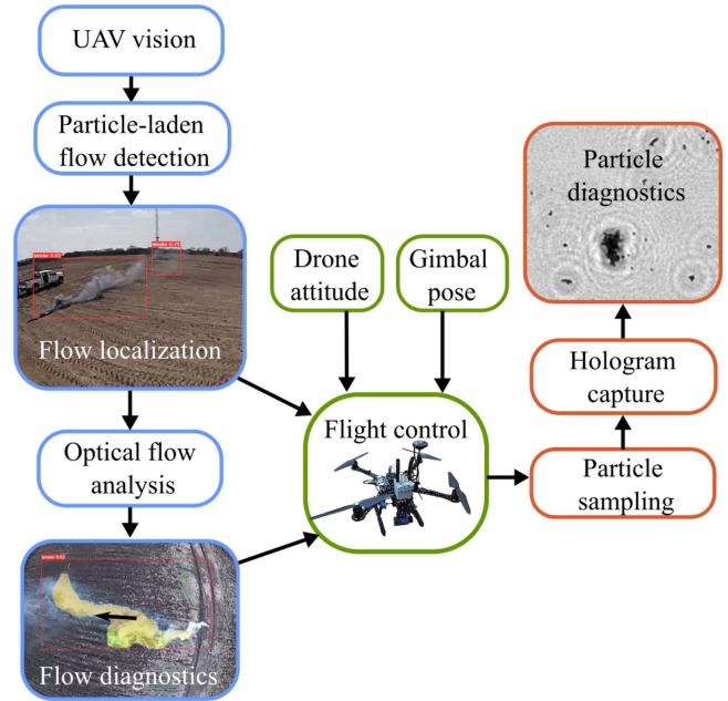
Fig. 1. Autonomous UAV operation workflow for enabling vision-based navigation and holographic imaging for in situ particle diagnostics.
