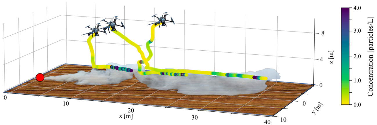
Fig. 9. Particle diagnostics data from the UAV-based DIH sensor during autonomous flight, showing a spatial map of particle concentration along the UAV sampling path, moving along heading determined by optical flow. Data are combined from three autonomous sampling sequences for the same smoke plume.
