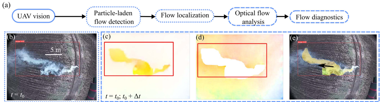
Fig. 3. Computer vision workflow for autonomous navigation of the UAV. (b) Shows an example of object detection for smoke plume, and (c)–(e) show optical flow process, including segmentation. (c) shows optical flow with the bounding box from object detection, (d) displays the segmented flow used for computing background motion, and (e) the final overlaid flow result with the bulk motion, computed from the segmented flow after background compensation, indicated with the black arrow.
