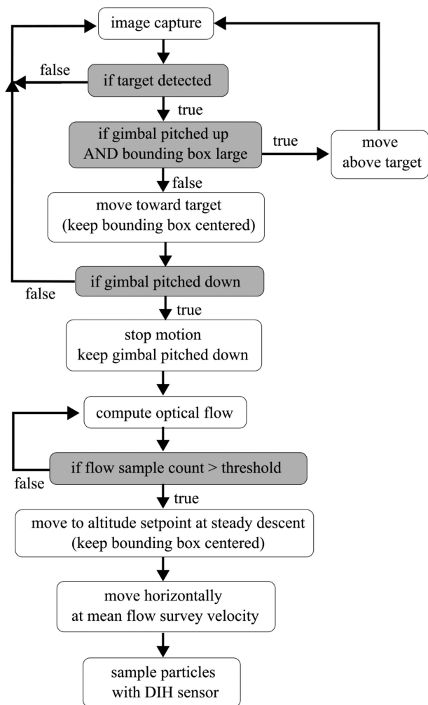
Fig. 4. Feedback control algorithm for approaching particle-laden flow, determining flow direction, and immersing UAV within particle-laden flow for optimal particle sampling.
