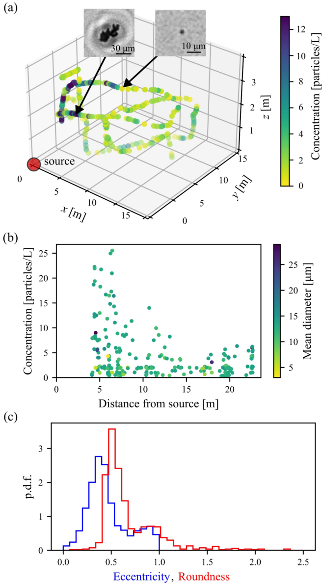
Fig. 8. Particle diagnostics data from the UAV-based DIH sensor. (a) Spatial map of particle concentration along the UAV sampling path, with the source of smoke emission show in red and the inset plots depicting reconstructed smoke particle holograms. (b) Concentration as a function of distance from the source, with marker color indicating mean equivalent diameter from each measurement location. (c) Probability density functions of eccentricity and roundness for all particles sampled.
