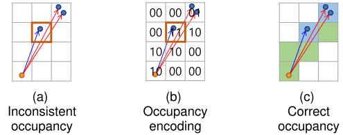
Fig. 5. Consistent voxel state. (a) In the orange voxel, three-ray intersections occur. The blue ray intersection labels the voxel as occupied because the ray endpoint is included in the voxel, whereas the red ray intersections label the voxel as free. (b) The voxel has two bits to encode the 00 (unknown), 01 (occupied), 10 (free), and 11 (free or occupied) states. (c) When there is an occupancy conflict, the occupied state (01) takes precedence over the free state (10). Thus, the orange voxel in (b) is colored blue (occupied) in (c) instead of green (free).
