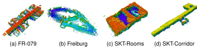
Fig. 7. PVM results of OctoMap-RT. The voxels are color-coded depending on the vertical height from the floor, and the dimension of each voxel is 10 \text{ cm}^3 .
