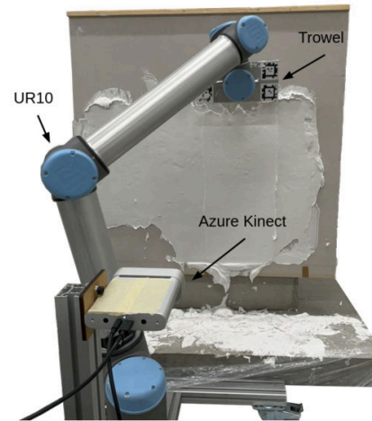
Fig. 5: The hardware setup constructed for physical experiments. The manipulator and camera are positioned in front of the work surface in the vertical setting.
