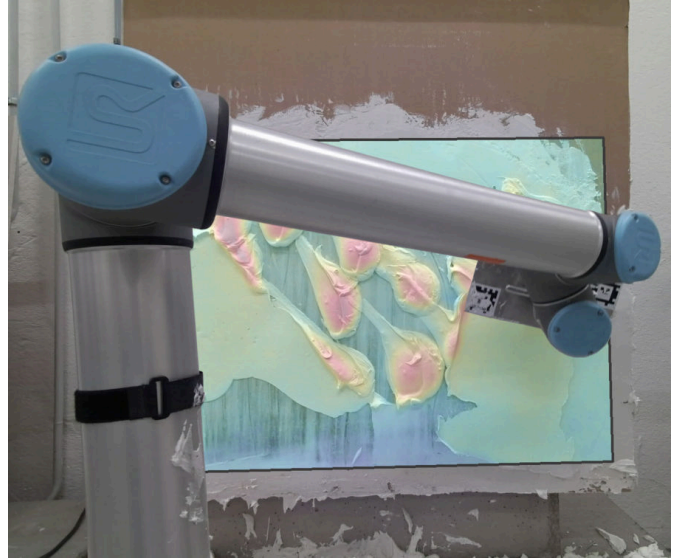
Fig. 1: A robotic manipulator is smoothing a surface with trowelling actions. The work area is marked, and the measured elevation is visualized with the overlaid color map.
