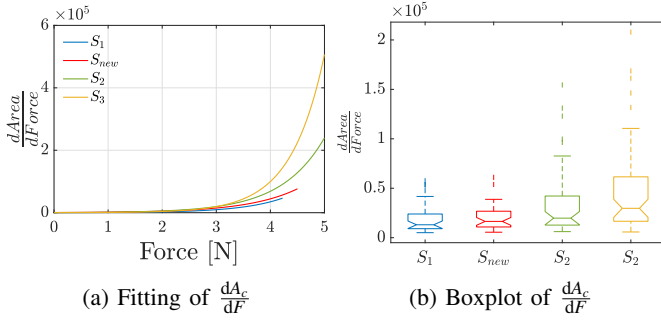
Fig. 8: S_{new} CASR discrimination based on the proposed model. Different specimens are color-coded, respectively, S_1 in blu, S_{new} in red, S_2 in green, and S_3 in yellow.
