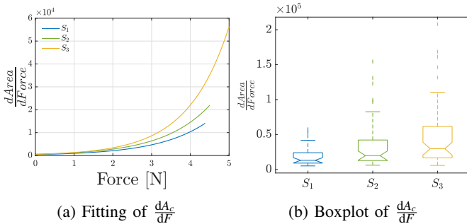
Fig. 6: CASR discrimination based on the proposed model. Different specimens are color-coded, respectively, S_1 in blue, S_2 in green, and S_3 in yellow.
