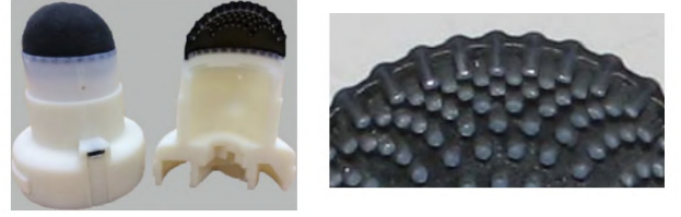
Fig. 1: Representation of TacTip internal structure [12]
