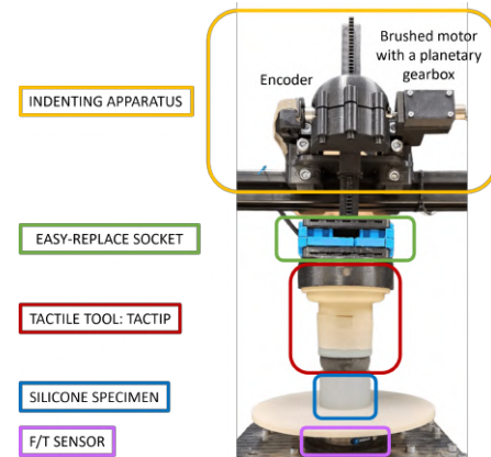
Fig. 3: The whole apparatus used both to characterize specimens' stiffness and in CASR validation experiment, composed of vertical moving support, the tactile tool, in the depicted case, the TacTip, fixed circular plate with an ATI force/torque sensor on the bottom.
