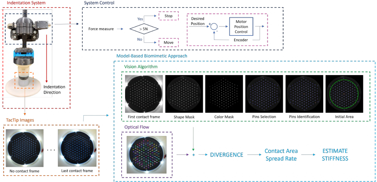
Fig. 4: Schematics describing the complete pipeline.
