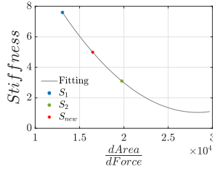
Fig. 7: \kappa_{S_{new}} estimation considering fitted model on \frac{dA_c}{dF} and \kappa Different specimens are color-coded, respectively, S_1 in blu, S_{new} in red, S_2 in green.
