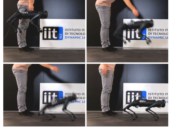
Fig. 1. Based only on proprioceptive measures, during a fall the proposed Landing Controller (LC) adjusts the limbs posture in order to drive the robot to stable standing configuration after Touch Down (TD), avoiding bounces, feet slippage and undesirable contacts with the ground.
