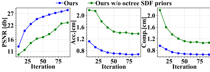
Fig. 9. Ablation study about octree SDF priors on one frame. We choose the first frame in Room0 of Replica [21] to evaluate how the mapping performance of the corresponding region changes with increasing optimization iterations.
