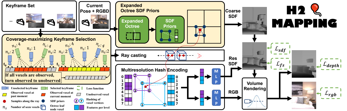
Fig. 2. The pipeline of H2-Mapping. Taking RGB-D image from sensors and pose from other tracking modules, we utilize an expanded octree SDF priors and multiresolution hash encoding to represent the scene from rough to detailed. Additionally, the proposed coverage-maximizing keyframe selection ensures quality in the edge regions.
