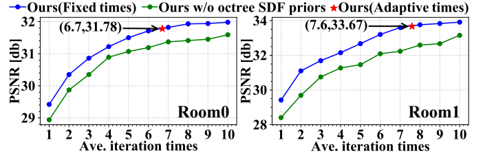
Fig. 10. Ablation study about the adaptive early ending and octree SDF priors on the entire data sequence. We compared changes in the PSNR [24] for different fixed iteration times in Room0 (left) and Room1 (right) of Replica [21]. The blue curve and green curve represent the results with and without octree SDF priors, respectively. The red star denotes the average iteration time and PSNR [23] using adaptive early ending.
