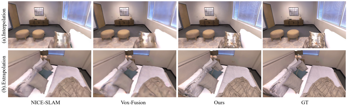
Fig. 7. Image rendering results on the Replica dataset [21]. (a) Rendering results from the input views (interpolation). (b) Rendering results from the novel views (extrapolation). The image rendered by our method has more high-fidelity details and rich textures, such as pillows and bed sheets
