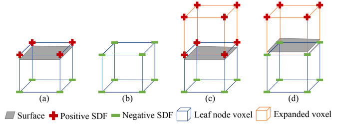
Fig. 4. The correct sign of SDF priors (a). And different situations when using voxel expansion (c,d) or not (b) as the surface is near the voxel’s boundary.
