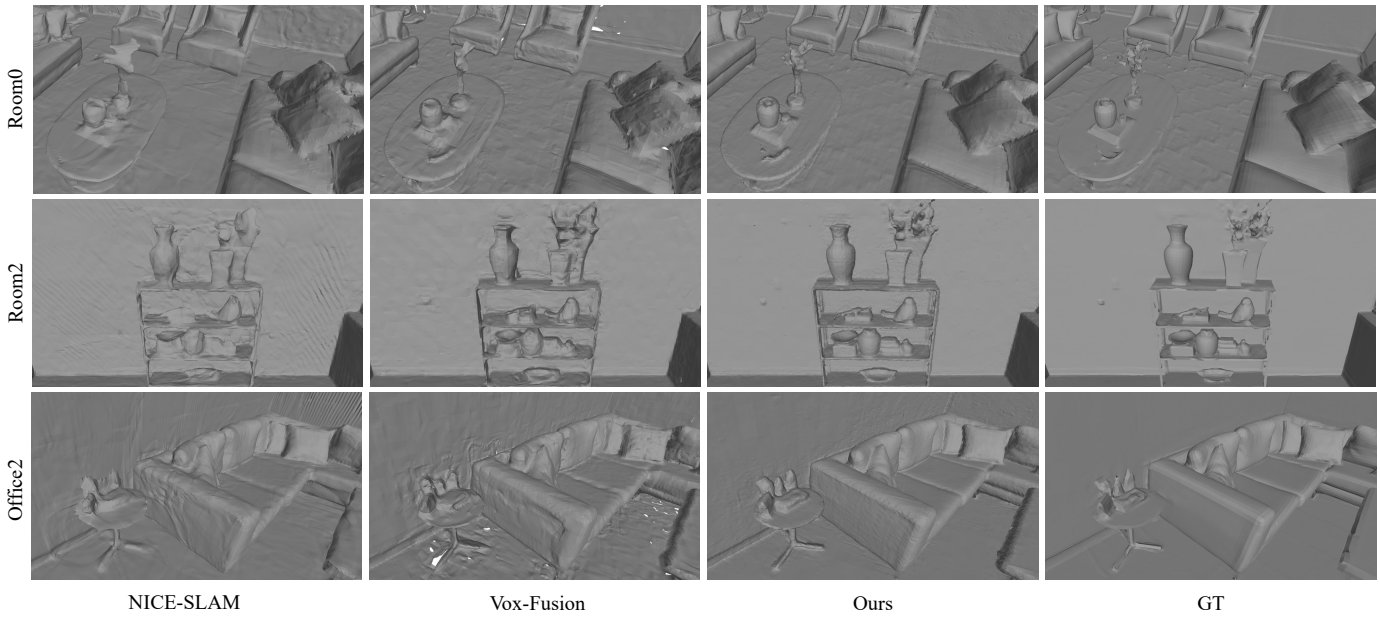
Fig. 6. Reconstructed mesh on the Replica dataset [21]. Our method closely approximates the ground truth mesh and can capture richer geometric details in small objects, such as chair legs and vases.
