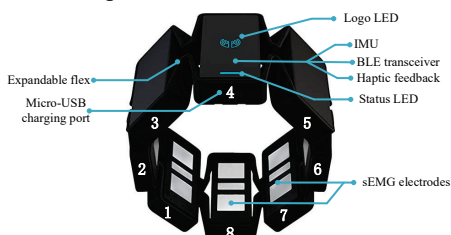
Figure 3. The Myo armband from Thalmic Labs.
