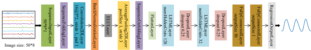
Figure 8. The schematic of the CNN-LSTM used on sEMG signals.
