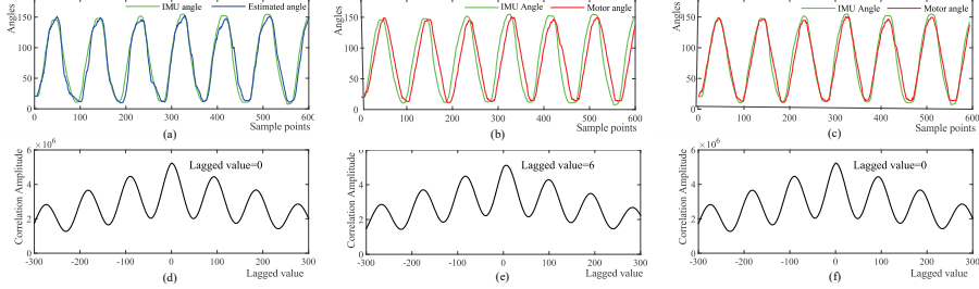
Figure 11. The online estimation and motor angle. (a) estimated angle (b) motor angle (c) motor angle without time lag (d) phase difference between the signal of estimated angles and IMU angles (e) phase difference between the signal of motor angles and IMU angles (f) phase difference between the signal of motor angles and IMU angles after time lag elimination.
