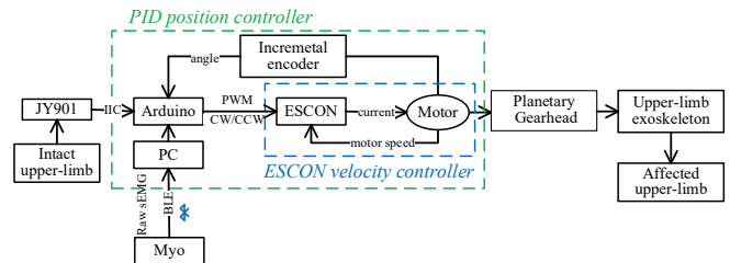
Figure 4. The overall design of the embedded system of the upper limb rehabilitation exoskeleton.
