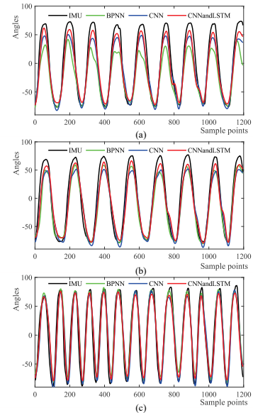
Figure 9. The offline angle estimation results under BPNN, CNN and CNN-LSTM. (a) angle estimation of subject 8 (b) angle estimation of subject 9 (c) angle estimation of subject 10.
