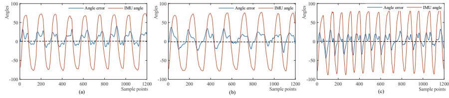
Figure 10 The angle error distribution between the estimation angle and IMU angle. (a) subject 8 (b) subject 9 (c) subject 10
