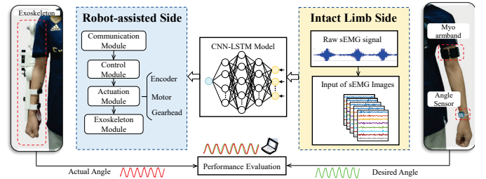
Figure 1. The overview of subject-independent estimation of continuous movements using CNN-LSTM for home-based bilateral upper limb rehabilitation system.
