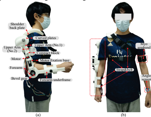
Figure 2. The upper limb exoskeleton device. (a) lateral view (b) front view.
