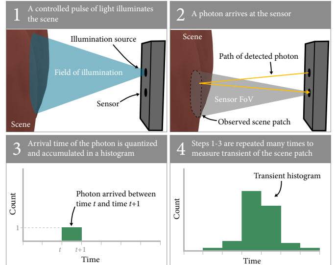
Fig. 1: The transient histogram is a temporal waveform which records the response of a scene patch when exposed to a pulsed light source. Presently available commodity sensors estimate the transient histogram through a repeated process.
