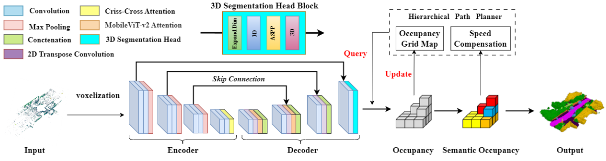
Fig. 3: SCONet: Lightweight Semantic Scene Completion Network. Our network employs a self-attention-driven U-Net architecture, featuring depthwise separable convolutions and segmentation heads, to perform efficient 3D scene completion and semantic segmentation.
