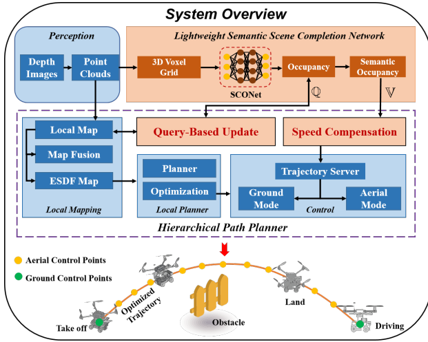
Fig. 2: The overview of our proposed Framework: AGRNav. \mathcal{Q} denotes that the free voxels in the grid map query and update their occupancy status from the predicted occupancy map. \mathcal{V} denotes that predicted semantics is turned into speed compensation.
