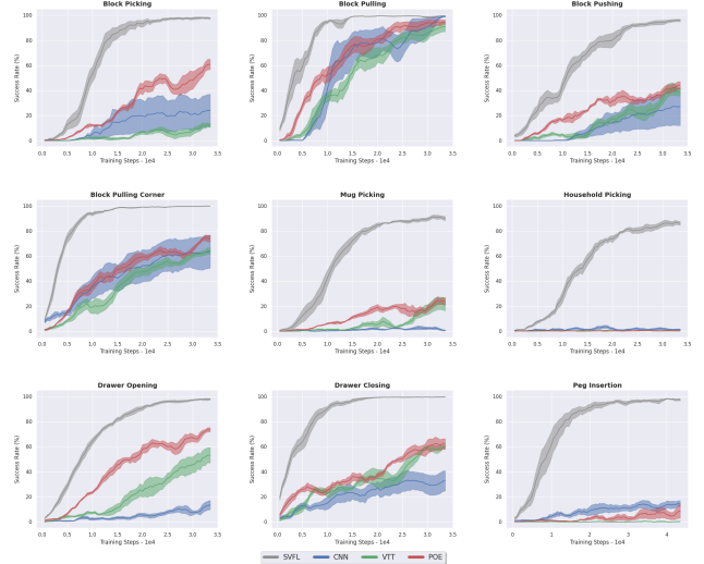
Fig. 4: Baseline Comparison. Comparison of SVFL (gray) with baselines. Greedy evaluation policy is shown in terms of success rate. In all of our experiments, results are averaged over 5 random seeds and the evaluation is performed every 500 training steps. Shading denotes standard error.
