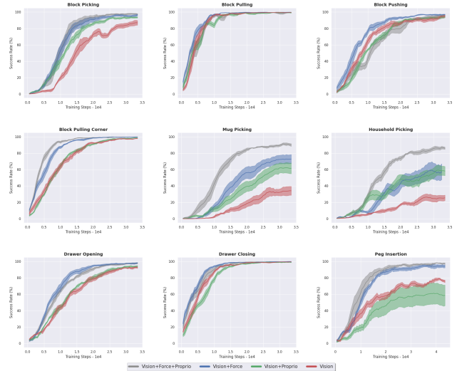
Fig. 5: Sensor Modality Ablation. Comparison of the full SVFL model (gray) to subsets of the data modalities.
