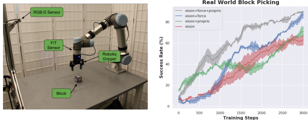
Fig. 7: On-Robot Policy Learning. (Left) Robotic setup. (Right) Comparison of the full SVFL model (gray) versus SVFL with subsets of the data modalities in the real-world on the Block Picking task. Results are averaged over 3 runs.
