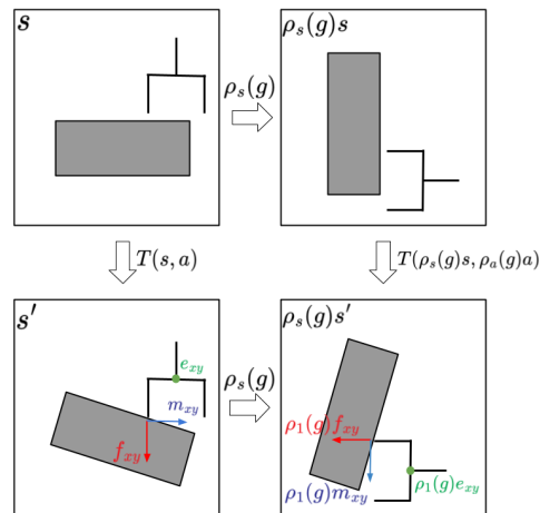
Fig. 1: Symmetries in Visual-Force Domains. An example of the O(2) symmetries in the visual-force policy learning problem. Note that the same rotational symmetries which apply to the image s also apply to the xy components of the force ( f_{xy} , m_{xy} ) and end effector state ( e_{xy} ).
