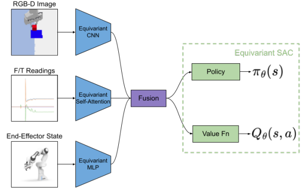
Fig. 2: Symmetric Visual Force Learning. SVFL combines visual, force, and proprioceptive feedback into a single joint-representation while respecting the symmetry inherent to each data modality.
