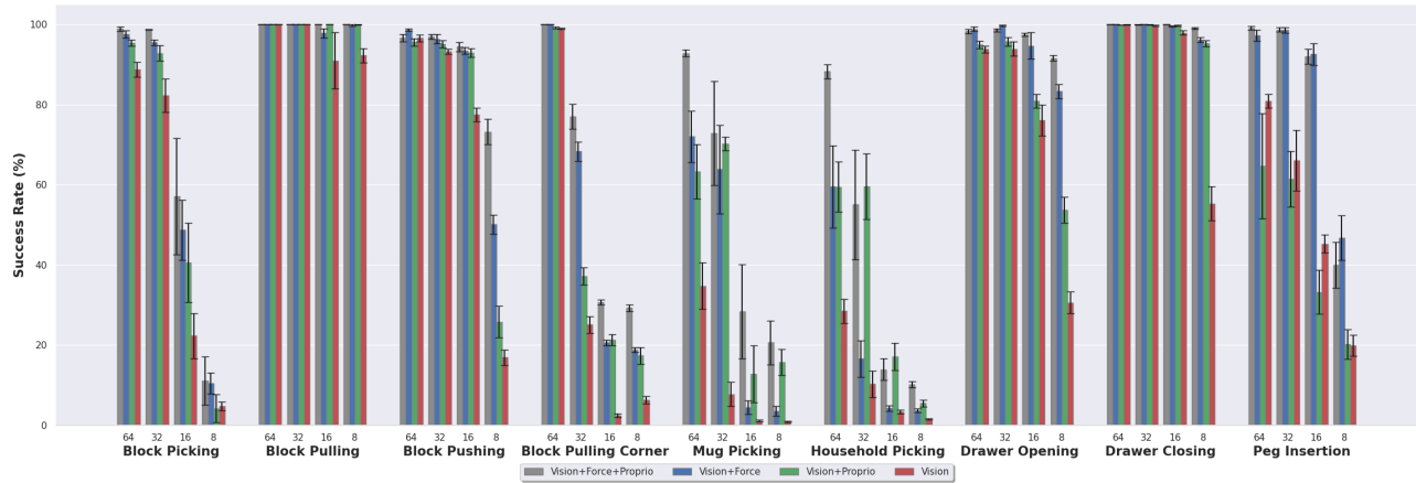
Fig. 6: Performance Under Degraded Visual Acuity. Comparison of the full SVFL model (gray) versus SVFL with subsets of the data modalities under visual acuity degradation. Performance is given after all models are trained to convergence.
