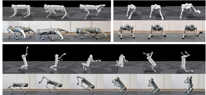
Fig. 6: The retargeted reference motions and the behaviors of the real-world robot. The reference motions are imperfect and physics-ignorant.
