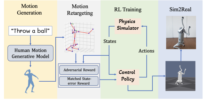
Fig. 2: Overview of the multi-phase method L anguage- G uided m otion c ontrol (LAGOON). To make a robot follow a language command such as “throw a ball”, we first generate a human motion using the motion generation model. Then the human motion can be retargeted to a robot skeleton that differs largely from humans. By introducing RL training, we train a robust control policy in the physics simulator. Finally, we deploy the control policy to the real-world robot.
