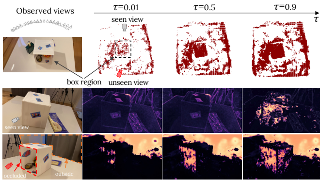
Fig. 5: Ablation study on the threshold \tau . Too small \tau causes low inferred pixel-wise uncertainties for rays casting through the unseen occluded scene regions, while too large \tau will destroy the reasonable uncertainty from the seen view.
