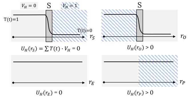
Fig. 3: The inferred pixel-wise uncertainty from our uncertainty field exhibits high value for rays that directly cast towards the occluded r_O or outside scene content r_P . T(t) represents the accumulated transmittance and will quickly decay to zero when hitting the surface (S).
