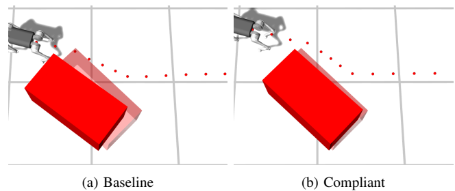
Fig. 6: The robot collides with a box weighing 2kg while following the command v_x^* = 0.4 , v_z^* = 0 , and \omega_y^* = 0 . The box’s initial position is indicated by the transparent area, and the robot’s path is traced by the dotted lines.
