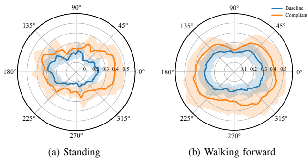
Fig. 4: Measurements of the decay time in seconds of a velocity disturbance in all horizontal directions while standing still (fig. 4a) or walking forward (fig. 4b) at 0.5 m/s. The solid line represents the average values from five policies trained with different seeds, with 10 runs each. The surrounding shaded area indicates the standard deviation.
