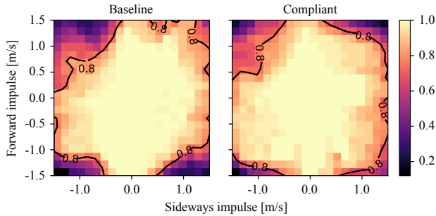
Fig. 2: Heatmaps depicting the push recovery success rates for both the baseline and the compliant controller. A contour line indicates the 80% success threshold
