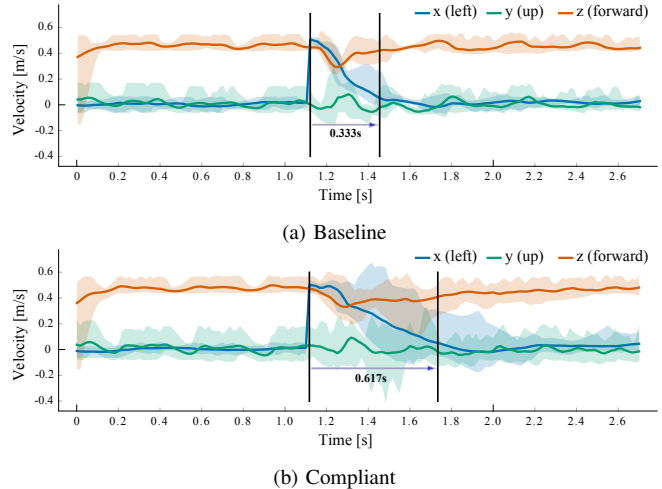
Fig. 3: The plots show the decay time of a velocity disturbance for the baseline (fig. 3a) and the compliant controller (fig. 3b.) The average is represented by the lines, with shaded regions indicating the minimum and maximum values of 20 individual runs of the same policy.
