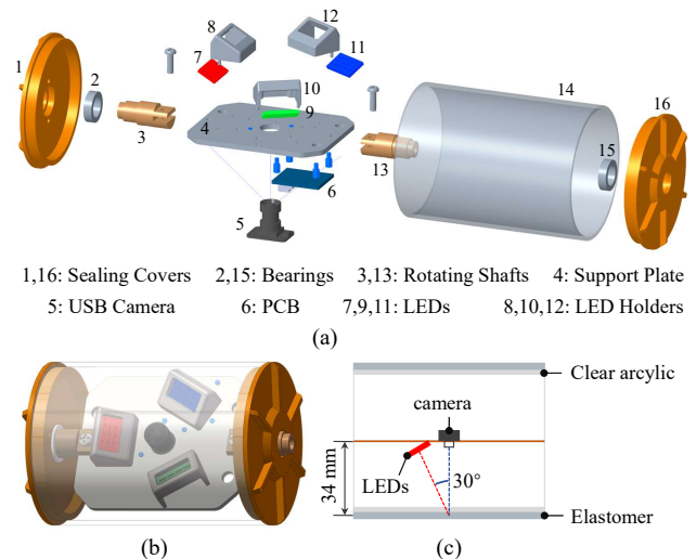
Fig. 2. Design of GelRoller: (a) An exploded view that reveals its internal components; (b) The assembled CAD model. (c) A structural sketch.
