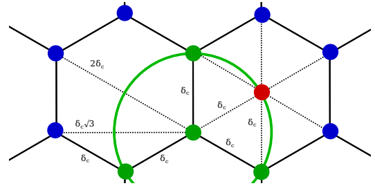
Fig. 3. Tesselation pattern used for covering Open space. Relay locations are depicted as small disks. The green disks denote a triple of relays connected with a communication range \delta_c illustrated as the green circle. The blue disks depict other relays in the resulting network \mathcal{N} . The red disk is a possible location at the center of the hexagon that can be used for the resulting 6-connected network.
