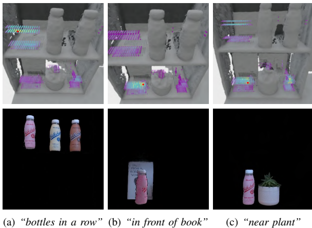
Fig. 6: Results for the three tasks on the shelf scene, with heatmaps (top row) and the highest-scoring renders (bottom).
