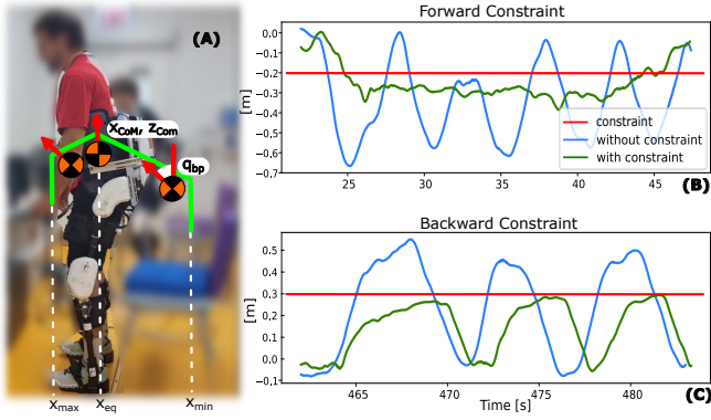
Fig. 2: Balancing constraint for the StS task: Fig. (A) shows the pose (position and orientation) of the CoM is constrained in both the horizontal and vertical planes; Fig. (B) shows how the position is constrained in the forward movement to avoid falling; Fig. (C) shows how the backward movement is constrained but still leaves the possibility of performing the StS task.
