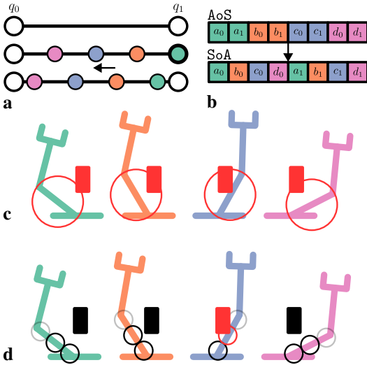
Fig. 2. Illustration of the “raked” motion validator for a two-link mechanism. a) The rake consists of evenly spaced configurations, which are “raked” backwards to achieve sufficient resolution. b) These configurations are computed in SoA form and c) checked in parallel. We use hierarchical sphere approximations of collision geometry to avoid unnecessary checks. d) When any collision is discovered at the lowest refinement level (in red), the entire check terminates (the last sphere in grey is skipped).
