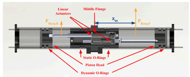
Fig. 3: Section-view of a single Buoyancy Engine.
