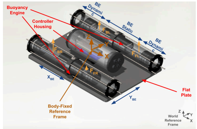
Fig. 2: Isometric view of the ReefGlider and relevant frames of reference.
