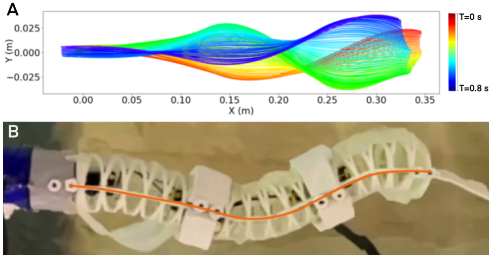
Fig. 7: (A) Clothoid representation of one swimming cycle. The color (ROYGBV) corresponds to the chronological progression of the tail. t = 0 s corresponds to red and t = 0.8 s corresponds to violet. (B) A snapshot of the physical model during the same locomotion experiment with a curve (orange) overlaid to indicate the tracked shape. In water snapshot taken at t = 0.06 s.
