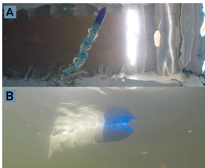
Fig. 8: (A) Robustness testing in Worcester Polytechnic Institute swimming pool and (B) Lake Quinsigamond. The robot is able to operate at depths of 0 to 2 m and can function with disturbances from wake and debris.
