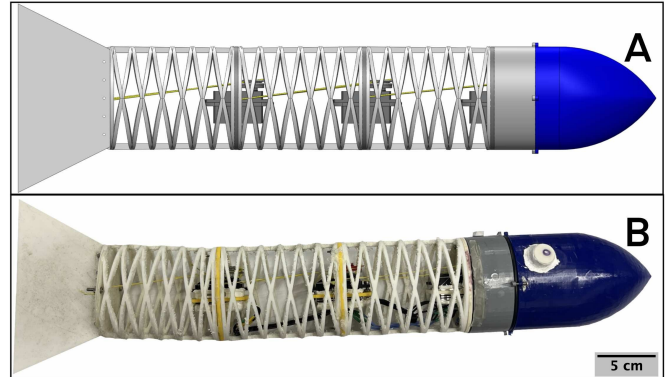
Fig. 1: (A) Cad model of the robot. (B) Physical robot with the addition of a latex skin on the wave spring tail. The three modules are connected together with individual motors to control their motion. The robot's body length was 0.496 m.
