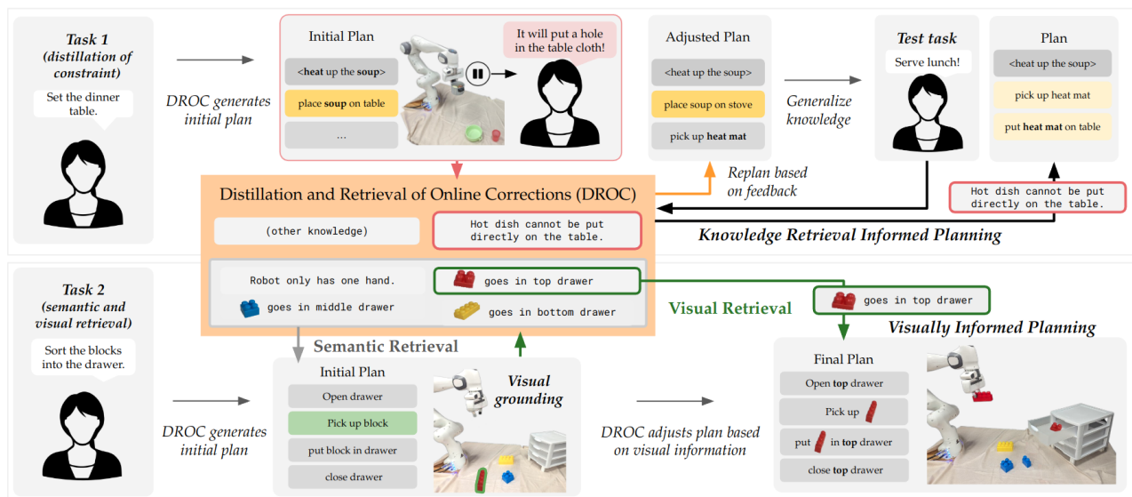
Figure 4: Illustrative examples for plan-level test cases. (1) upon interruption, DROC responds to correction by identifying it is a plan-level error and replanning, and distills the constraint for future tasks; (2) given a task with ambiguity, DROC retrieves past experiences base on semantic and visual similarities.
