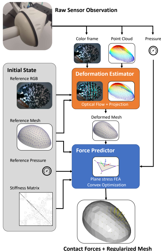
Fig. 1: A summary of the force estimation pipeline. An RGB image and point cloud from the bubble sensor are used to estimate the 3D deformation relative to a reference configuration. We construct a finite element model of the bubble to predict forces from observed deformations and pressure changes. A convex optimization problem combines the physics model and camera observations, giving contact force estimates and regularizing the raw observations.
