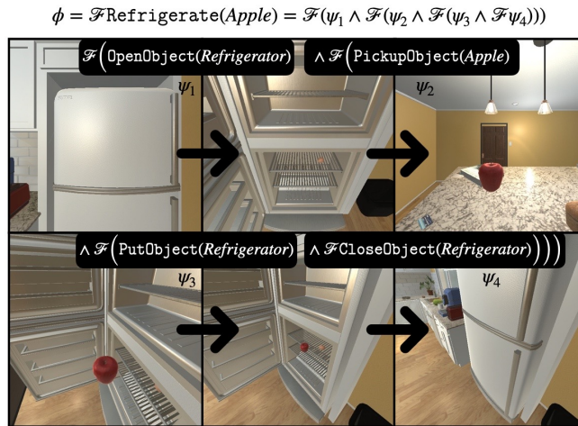
Fig. 1: Cook2LTL in AI2-THOR [21]: The robot is given the instruction Refrigerate the apple . Cook2LTL produces an initial LTL formula \phi (top left); then it queries an LLM to retrieve the low-level admissible primitives for executing the action; finally it generates a formula consisting of 4 atomic propositions ( \psi_1, \psi_2, \psi_3, \psi_4 ) that provide the required task specification and yield these consecutive scenes.
