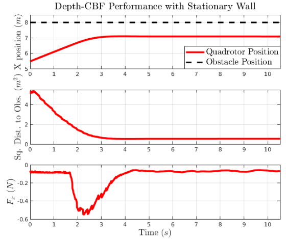
Fig. 10. Simulation results for the quadrotor: in plot 1, we see the x position of the quadrotor with respect to the wall, in plot 2 the squared distance from the quadrotor to the wall, and in plot 3 the x component of the force vector from the Depth-CBF-QP optimization. We observe that the Depth-CBF enables the quadrotor to smoothly avoid collision with the wall.
