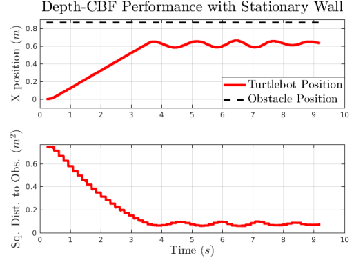
Fig. 6. TurtleBot trajectory and squared distance to obstacle in the presence of a stationary wall in hardware. The Depth-CBF controller enables the TurtleBot to stop short of collision with the wall. The authors interpret the “steps” and oscillation visible in the value of the squared distance as a byproduct of the low refresh rate of the lidar.
