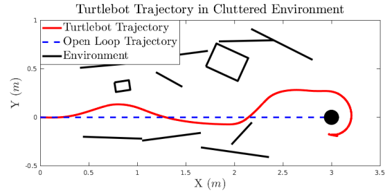
Fig. 9. The trajectory of the TurtleBot through the hallway in hardware. The black lines and boxes represent the obstacles depicted in Figure 8. Using the Depth-CBF, the TurtleBot successfully avoids the obstacles and navigates to the end of the hall with no information other than a straight open-loop trajectory.
