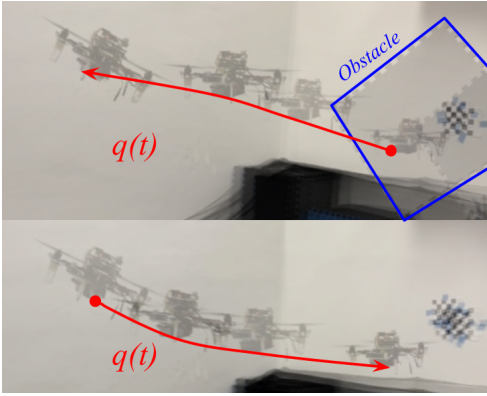
Fig. 11. Quadrotor hardware test: using the Depth-CBF, the quadrotor is able to successfully avoid a moving obstacle which is brought towards it at a constant velocity. When the obstacle is removed, the quadrotor returns to its initial position.
