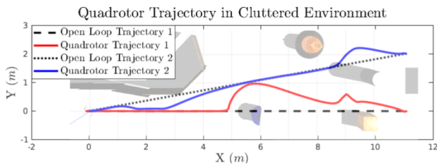
Fig. 13. The trajectories of the quadrotor through the simulated cluttered environment. The quadrotor is successfully able to navigate around the environment without collision for both of the open loop trajectories.
