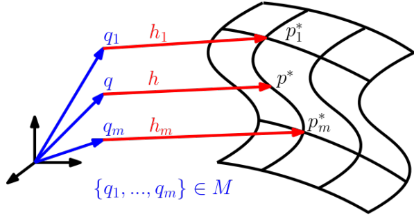
Fig. 3. By sampling the closest point in P to the system in a region surrounding the position q , we gain a local model of the barrier function.
