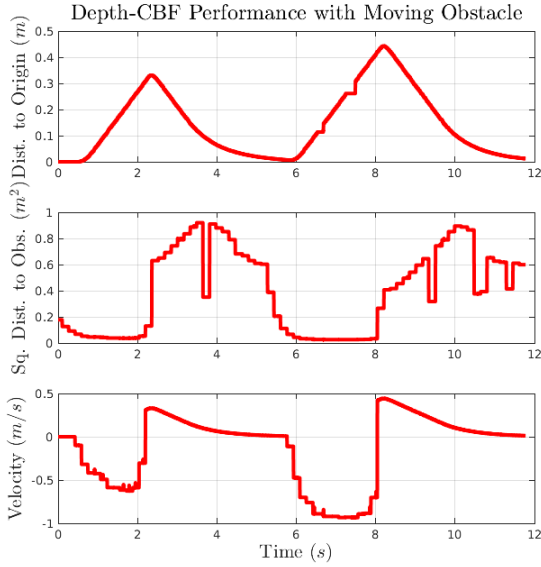
Fig. 7. Depth-CBF performance on the TurtleBot hardware in the presence of a moving obstacle. An obstacle is brought towards the system and removed, and the TurtleBot is able to successfully avoid the moving obstacle.
