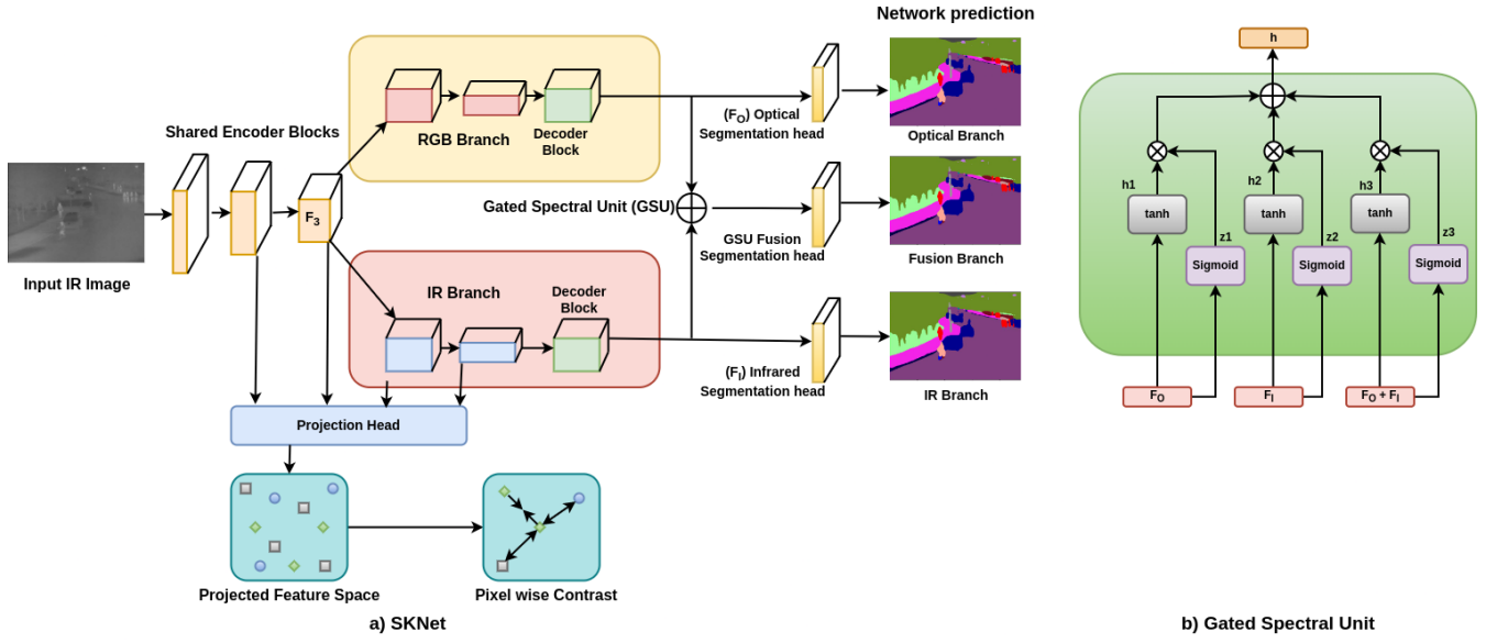
Fig. 2. Spectral-based knowledge distillation network (SKD-Net) architecture. a) The first three encoder blocks are shared between EO and IR branches. The output of the decoder block of the two branches is fed into GSU for feature fusion. Pixel-wise contrastive loss is used for features from the four encoder blocks (two from shared and two from the IR branch). b) Gated Spectral Unit takes three inputs from the EO branch, IR branch, and pixel-wise addition of the features of the two branches and outputs a single feature map.
