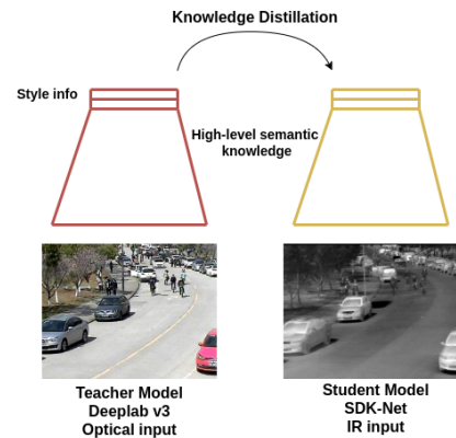
Fig. 1. Proposed knowledge distillation framework encourages SKD-Net to transfer semantic knowledge between optical and IR modalities.
