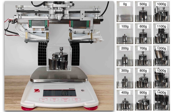
Fig. 7: Experimental setup for sensing different weights. (Left) For each of 7 pre-defined grasp strengths, the gripper makes 3 attempts to grasp a box filled with weights. A digital scale confirms a successful lift-off. (Right) The experiment is repeated with 15 weights from 0 to 1400 g.
