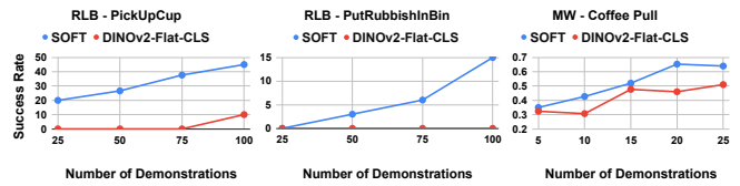
Fig. 4. Success rate of different methods as a function of the number of demonstrations.
