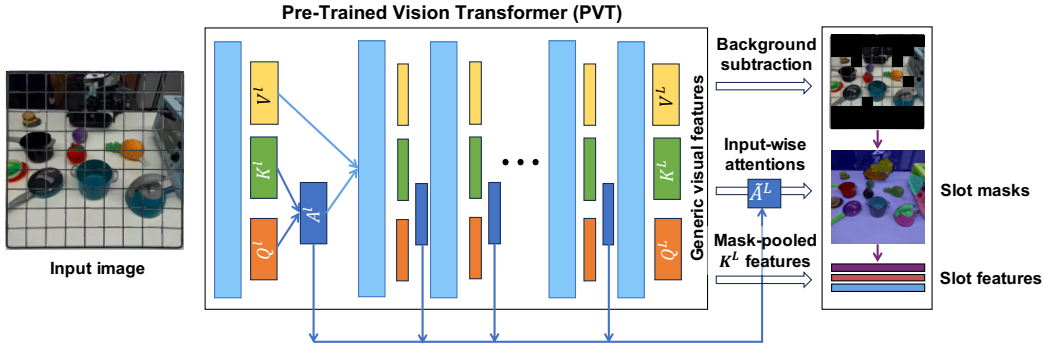
Fig. 2. \text{SOFT}(\cdot) provides a wrapper around any pre-trained vision transformer model PVT. Relying on nothing other than the activations and attentions throughout PVT, \text{SOFT}(\cdot) offers an alternative representation inference procedure to the standard last-layer activations. The resulting \text{SOFT}(\text{PVT}) representation is an object-centric image representation, suitable for off-the-shelf usage in robotic control tasks. V^l , K^l and Q^l represent the value, key and query of attention layers at layer l .
