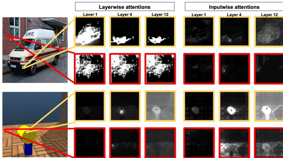
Fig. 1. Visualizing attentions for two images from ImageNet and Shapestacks. On each image, we consider a foreground patch (yellow) and a background patch (red). Attentions a_{ii} for each patch towards itself are zeroed out to identify the patch in attention images. Layerwise attentions at various DINO layers (left) reveal little information at higher layers, so we instead compute inputwise attentions (right) using attention flow.
