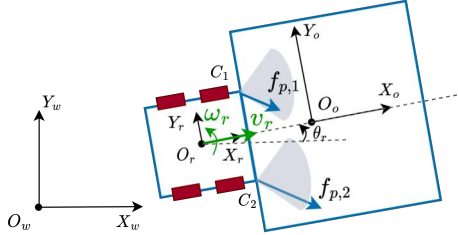
Fig. 4. Schematic of the robot-object pushing system.
