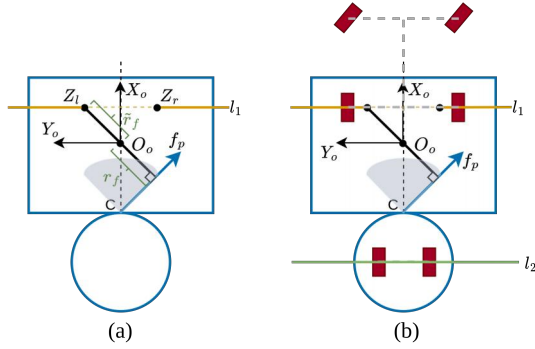
Fig. 2. Illustration of the possible center of rotation. The circle and the rectangle represent the robot and the object in a 2D plane. The grey area and the blue arrows respectively indicate the friction cone and its edges. The orange line indicates the set of rotation centers of the object under stable push. While the green line is the robot's common left and right wheel axis and the line of its possible rotation centers. In (a), the object is pushed by an omni-directional pusher with a point contact. The set of its possible rotation centers lies on the orange line. In (b), the object is pushed by a nonholonomic robot with its rotation centers on the green line. However, there is no overlap between the possible rotation center of the wheeled robot and the object under this contact configuration. The red bricks, connected by grey dashed lines, represent the wheels of a car model in Dubin's car problem.
