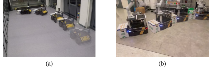
Fig. 1. The wheeled mobile robots (Clearpath Husky and Boxer) push a paper box to a goal location and to track a reference path, respectively. Transparency of the robots and box indicates their movement.
