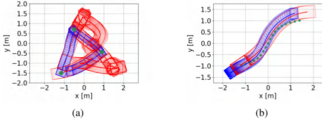
Fig. 8. Stable pushing across different scenarios. (a) Push an object around the room. (b) Path following while engaging in stable pushing. The red and blue curves represent the trajectories of the robot and the pushed object, respectively. The reference waypoints are marked in green. In (b), a sponge sheet is stuck to the box to augment friction in the robot-object interaction, where k' = -k'' = 0.4 . For detailed information, we direct readers to our accompanying video.
