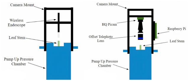
Fig. 11: Diagram showing how the custom-made mount and camera setups (left: endoscope, right: high quality Picamera) are mounted onto the manual pump-up chamber. The mounting onto the 600D nitrogen gas pressure chamber follows a very similar manner and is not shown here for brevity.
