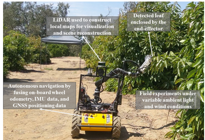
Fig. 3: The agricultural robot used in this work for robotic assessment of a crop’s need for watering.
