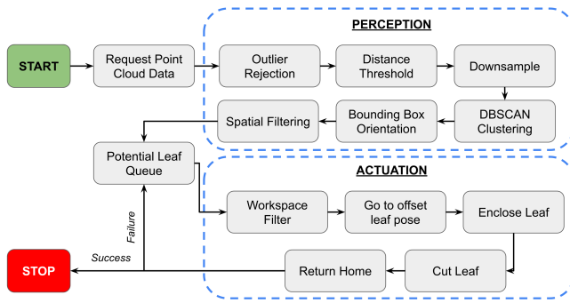
Fig. 7: Our approach for autonomous leaf extraction integrates perception and actuation. Point cloud data are processed at runtime to segment leaves and add leaf candidates into a queue. Candidate leaves are then passed to the robot arm and end-effector. If a cut is successful, the routine ends but if not, the next leaf in the queue is requested and the process repeats.
