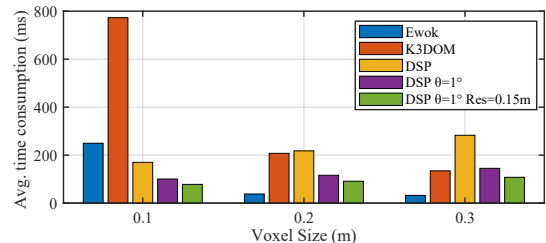
Fig. 13. Time consumption of different maps on Jeston Xavier NX.
