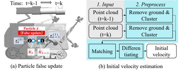
Fig. 4. (a) Illustration of the particle false update problem and (b) the initial velocity estimation procedures. In subfigure (a), a dynamic obstacle (a mobile robot) moves rightwards from t = k - 1 to t = k . At t = k - 1 , a measurement point z_{k-1}^{(1)} , on the right side of the obstacle, is observed. With z_{k-1}^{(1)} , a particle with state \tilde{\mathbf{x}}_{k-1} is generated in the particle birth step (Section V-C). Since z_{k-1}^{(1)} doesn't provide velocity, the commonly used way is to give \tilde{\mathbf{x}}_{k-1} a random velocity, e.g., a velocity to the left. At t = k , following the CV model, \tilde{\mathbf{x}}_{k-1} moves to \tilde{\mathbf{x}}_k . Since the particle's velocity is the opposite to the obstacle's velocity, this particle should belong to noise and its weight should be decreased in the update procedure at k . However, due to the large size of the robot, another measurement point z_k^{(2)} , close to \tilde{\mathbf{x}}_k , may be observed at k and falsely increased the weight of the particle in the update step. We call this problem the particle false update. Note the problem also exists in modeling large-size static obstacles and is more frequent when multiple dynamic and static obstacles exist, in which case particles generated from one obstacle may be falsely updated with the measurement from another obstacle.
