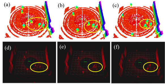
Fig. 17. Snapshots of mapping with the point cloud from Lidar. The top row shows the DSP map, and the bottom row shows the point cloud data. The yellow ellipses outline three pedestrians. In (d) and (e), the two pedestrians on the right are occluded or partially occluded but are clearly shown in the map. In (f), the pedestrians are detected by the Lidar again.
