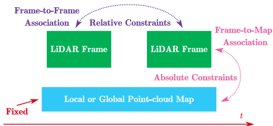
Fig. 1. An illustration of the frame-to-frame and the frame-to-map association in LiDAR navigation.
