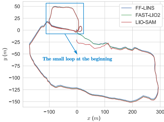
Fig. 7. The trajectories on the R3LIVE-hkust_campus_01 dataset.
