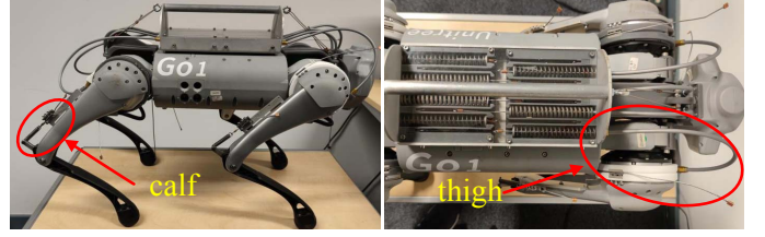
Fig. 9: Two views of the E-Go robot, a Unitree Go1 robot enhanced with springs acting in parallel to all the twelve joints. The springs acting in the sagittal plane for the E-Go robot are highlighted.
