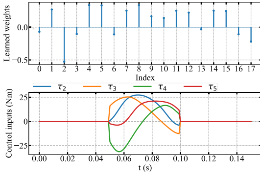
Fig. 6: An example of the learned weights (top) and resulting torque inputs (bottom) obtained when using the truncated Gaussian kernels.
