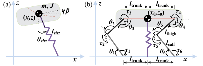
Fig. 2: The TSLIP at touchdown (a) and the CSBD anchor model in homing configuration (b). In (b).
