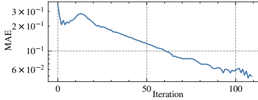
Fig. 7: The evolution of maximal absolute error when using the continuous learning variation of fILC.
