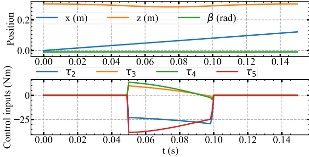
Fig. 3: Optimization results of the CSBD model with springs. We show both the evolution of the system and the control action for one single stride.
