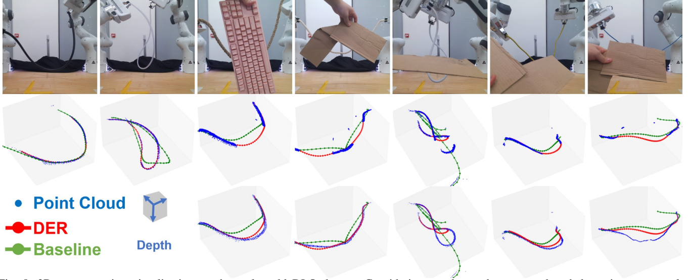
Fig. 8: 3D reconstruction visualization on the real-world DLO dataset. Considering we do not have ground-truth keypoints, we overlay reconstructed DLOs on unoccluded point cloud in the last row to show connection and fitness.
