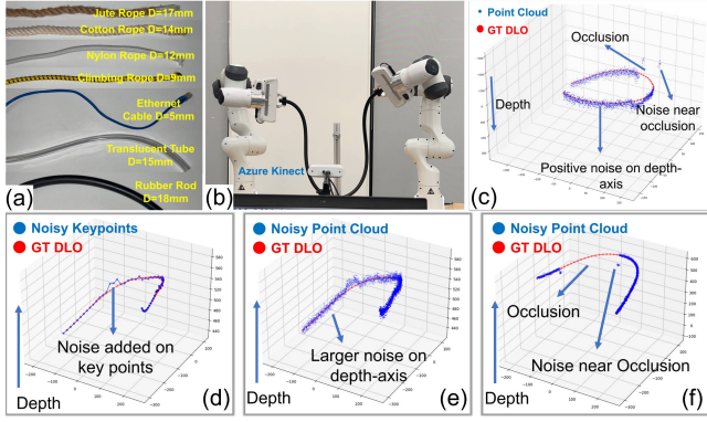
Fig. 5: Data Collection. (a) Seven DLOs used in the experiments. (b) Real-world DLO data collection with two Franka arms and an Azure Kinect. (c) Synthetic DLO dataset generation, where the red points are the DLO ground-truth, and the blue points are synthetic point cloud points created by adding different types of noise to the DLO ground-truth. (d) Ground-truth DLO with keypoints and keypoints with added noise in the depth-axis. (e) Gaussian noise added in all directions, but larger in the depth-axis. (f) Random occlusion and noise added to the DLO point cloud near occlusion.
