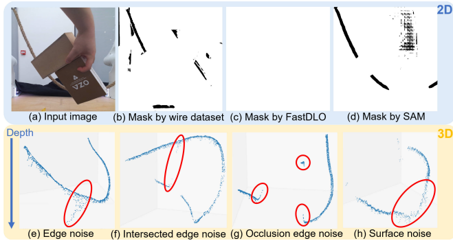
Fig. 2: Several DLO perception challenges. Top: Low-quality DLO segmentation mask from current approaches. (a) An RGB image of an occluded jute rope. (b) A segmented mask using a segmentation model trained on the wire dataset [10]. (c) A segmented mask using FastDLO [12] (no DLO is detected in this case). (d) A segmented mask using SAM with the text prompt “rope” [18]. Bottom: Noisy points caused by the flying pixel issue in the DLO point cloud. (e) Flying pixels between the edge of the DLO and the table. (f) Flying pixels between two self-intersecting parts near each other. (g) Flying pixels between the DLO and the occlusion. (h) Noisy point cloud of reflective DLO surface.
