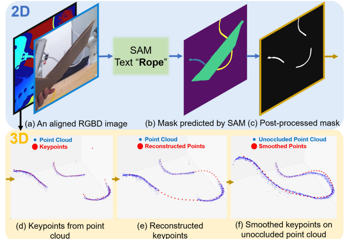
Fig. 1: Our 3D DLO perception pipeline.
