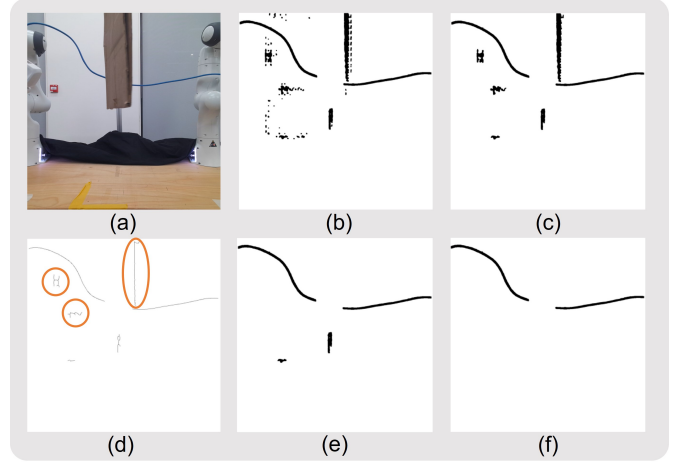
Fig. 3: Post-processing the DLO masks from SAM. (a) is the image of an occluded Ethernet cable. (b) is the mask directly generated by SAM with a text prompt rope . The black area is the DLO mask. (c) is the mask by removing all components whose area is below a certain threshold. (d) is the skeleton extracted from (c), where we circle all irregular skeletons. (e) is the mask that removes all components whose skeletons have irregular numbers of ends and conjunctions. (f) is the final post-processed mask by removing thick or too thin width components.
