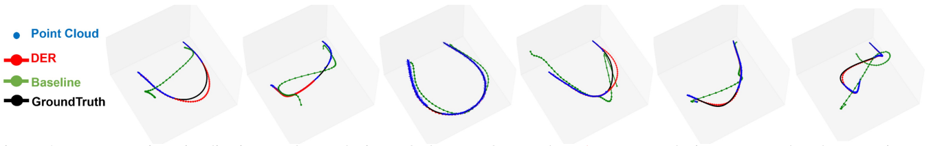
Fig. 7: 3D reconstruction visualization on the synthetic DLO datasets. Our result, red curves overlaying on ground-truth curves in most cases, outperforms the baseline model with more correct connection and fitting.
