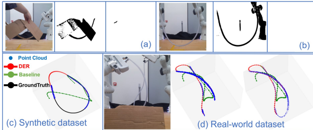
Fig. 10: Failure cases; (a), (b) on post-processing where the DLO mask is removed. (c), (d) on 3D reconstruction where the connection is incorrect.
