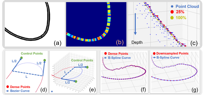
Fig. 4: The reconstruction method. (a) the mask and the keypoints found using morphological operations. (b) the result of K-Means clustering on the 2D mask, where each color represents the mask pixels in the same cluster, and the cluster center is the keypoint in (a). (c) a comparison figure where lightgreen points are the median of all points in the same cluster (top 100%), red points are the median of those points having the top 25% smallest depth, and blue points are the original 3D points selected by the segmentation mask. Bottom: (d) and (e) demonstrate using a Bezier curve to connect the two components of the DLO in 2D and 3D. (f) a DLO showing both the dense directly reconstructed 3D keypoints (red), and interpolating B-Spline (blue curve). (g) a DLO showing the blue interpolating B-Spline from (f), with sparse downsampled B-Spline points (red).
