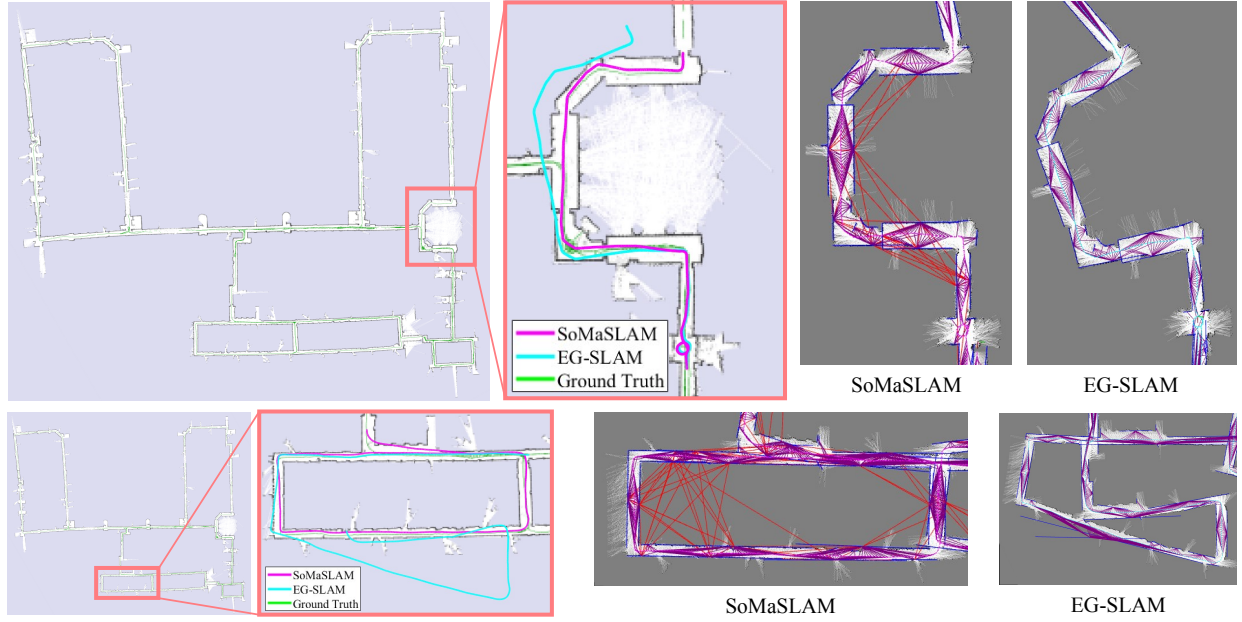
Fig. 8. Pose comparison of SoMaSLAM (magenta), EG-SLAM (cyan), and the ground truth (green) on the MIT Killian dataset (4pts). Landmark graphs of SoMaSLAM and EG-SLAM are on the right. The landmark-landmark constraints (red edges) enhance overall mapping accuracy, showing the near-perfect estimated trajectories of the proposed SoMaSLAM.
