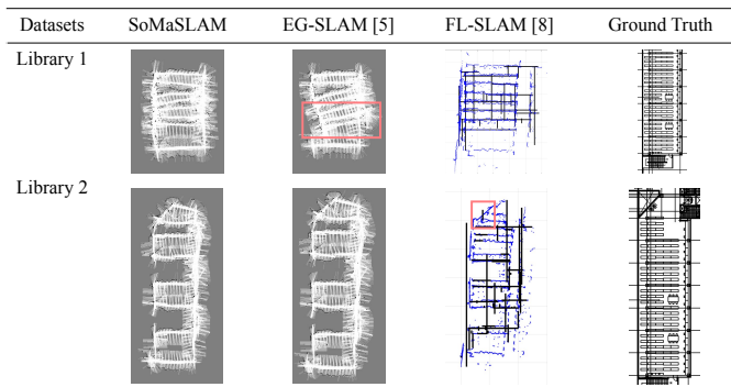
Fig. 11. Library 1 and Library 2 dataset (4pts) results with SoMaSLAM, EG-SLAM [5], and FL-SLAM [8]. FL-SLAM plots the point cloud (blue) and creates wrong walls (black). EG-SLAM struggles to map Library 1, and FL-SLAM fails to map the diagonal walls present in Library 2.
