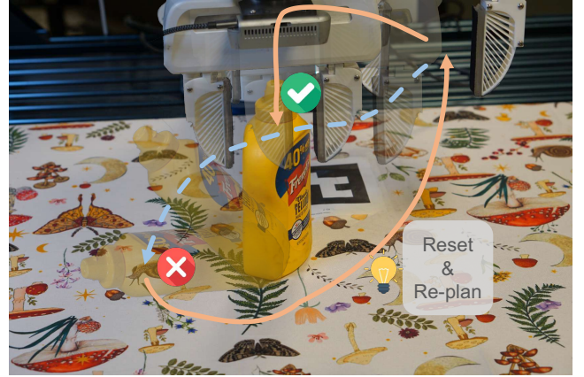
Fig. 3: DAgger Data Collection in Simulation. With privileged information provided by simulation, we can record and relive the failure cases during rollouts and generate corrective data for policy adaptation.
