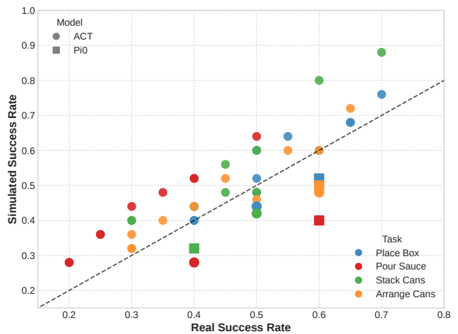
Fig. 9: Visual Benchmarking with FR3. We roll out various policies in both real and sim. We intentionally use different policies and data sizes to show positive correlations of sim-real performance regardless of the quality of the policies.
