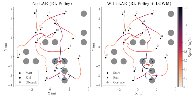
Fig. 4: Representative trajectory comparison. Left: base RL policy (no LAE), which collides with obstacles. Right: RL policy with LAE, which avoids collisions while remaining identical to the base policy in safe regions and still reaching the goals. Trajectories are coloured by speed. Numbers denote quadrotor index.
