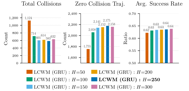
Fig. 6: Effect of editing horizon H for LAE with LCWM (GRU).
