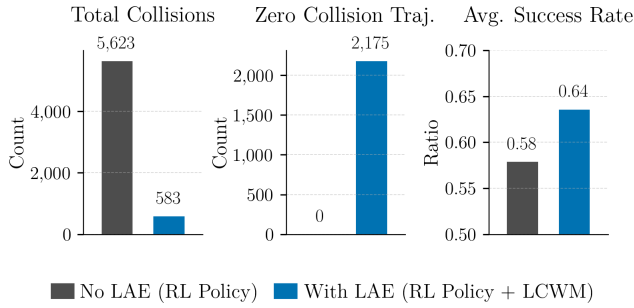
Fig. 3: Quantitative comparison of the base RL policy with and without LAE on 2,600 environmental configurations. We report total collisions, zero collision trajectories, and average success rate.
