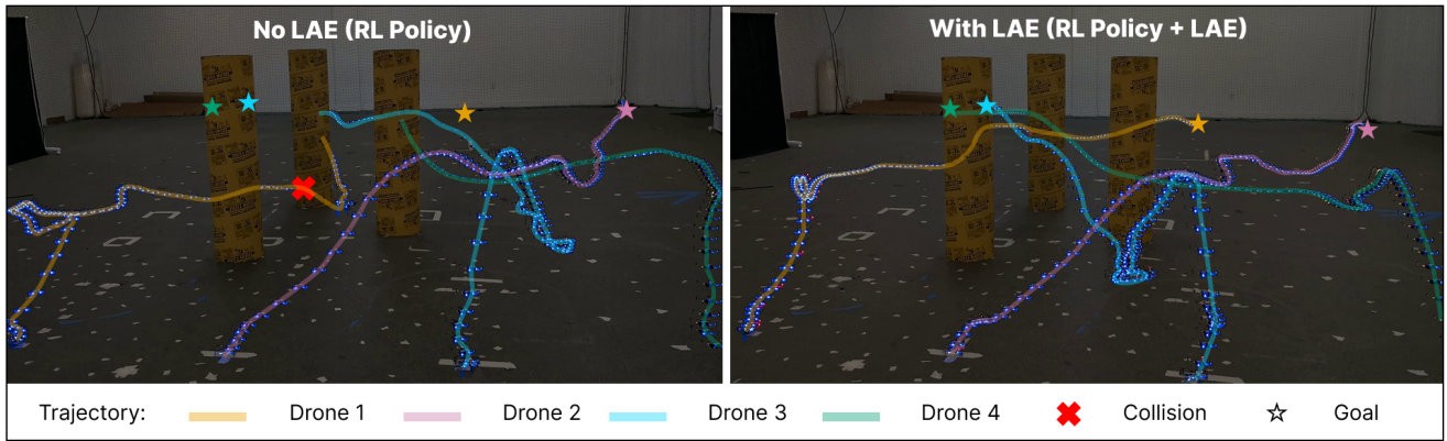
Fig. 7: Real-world deployment with 4 Crazyflie quadrotors navigating among cylindrical obstacles. Left: with the baseline RL policy, Drone 1 collides with an obstacle, leading to task failure. Right: with LAE enabled, all drones avoid collisions and reach their goals.
