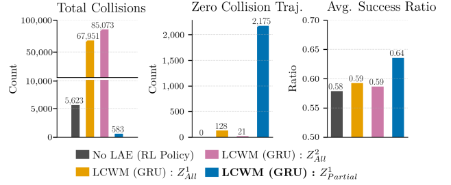
Fig. 5: Choice of Z_t : Comparing Z^1_{All} , Z^2_{All} , and Z^1_{Partial} . Z^1_{Partial} offers the best safety–performance trade-off.
