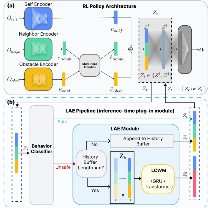
Fig. 2: Overview of LAE integrated on a pre-trained multi-quadrotor navigation policy. (a) RL policy architecture : observations are encoded and fused via multi-head attention to produce intermediate latent activations ( Z^1, Z^2 ), which serve as candidates for Z_t . (b) editing pipeline : a behavior classifier evaluates latent activation Z_t and forwards it unchanged if safe, or routes it to the editing module if unsafe. The module maintains a short history buffer and, once filled, invokes the LCWM to generate a surrogate Z'_t that replaces the unsafe latent activation Z_t .
