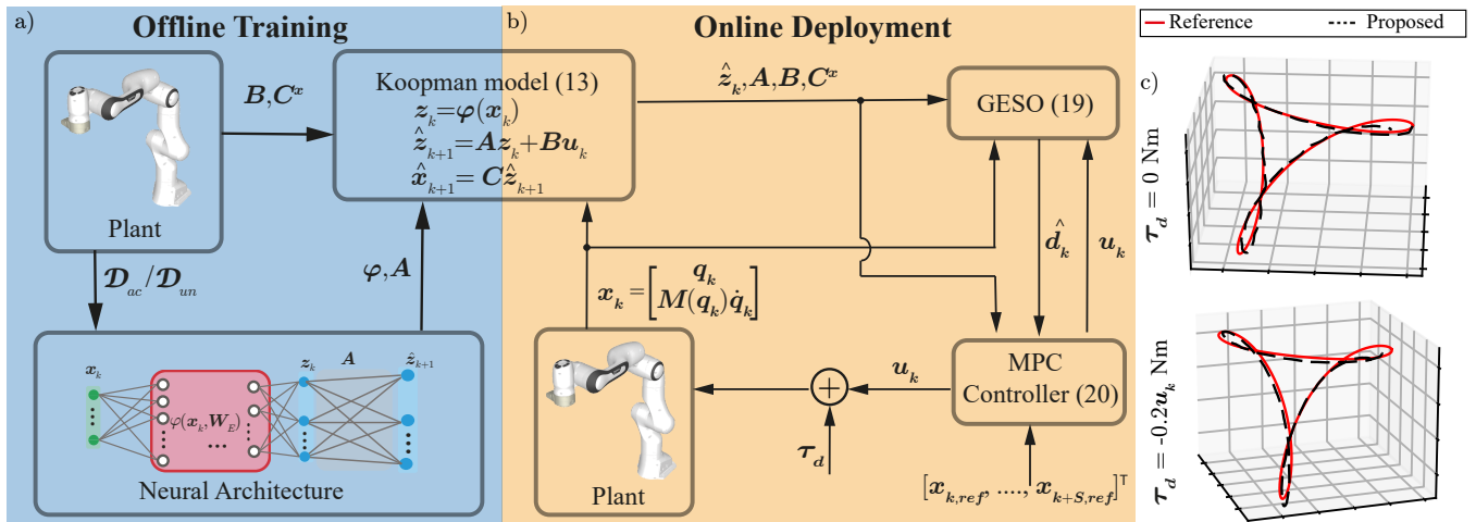
Fig. 1. Framework of the proposed momentum-based Koopman-MPC-GESO architecture depicting a) model training, b) control framework, and c) trajectory tracking results.
