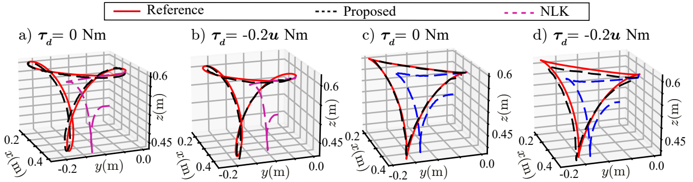
Fig. 4. Experimental results for trajectory tracking with the FR 3 manipulator, a,c) without, and b,d) with external disturbances.
