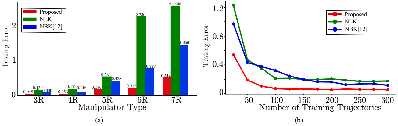
Fig. 2. Predictive performance comparison for the proposed scheme with Nominal Linear Koopman (NLK) and Nominal Bilinear Koopman (NBK) [12]. Testing errors across a) different manipulators, and b) different sizes of training datasets for a 4R manipulator.
