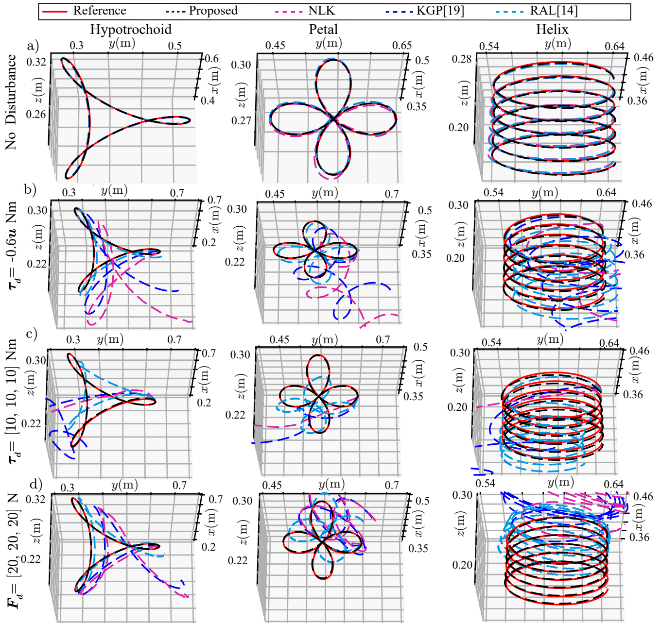
Fig. 3. Tracking performance comparisons for a 3R serial manipulator with a) no disturbance, b) actuator fault ( \tau_d = -0.6u Nm), c) constant disturbance torque ( \tau_d = [10, 10, 10] Nm), and d) constant end-effector load ( F_d = [20, 20, 20] N).
