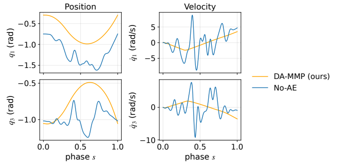
Fig. 7. Effect of the autoencoder on trajectory generation. Shown are positions ( q_1, q_3 ) and velocities ( \dot{q}_1, \dot{q}_3 ) of two representative joints. Our method (orange) produces smoother and more coherent trajectories, whereas the no-AE variant (blue) exhibits irregular and oscillatory motions.
