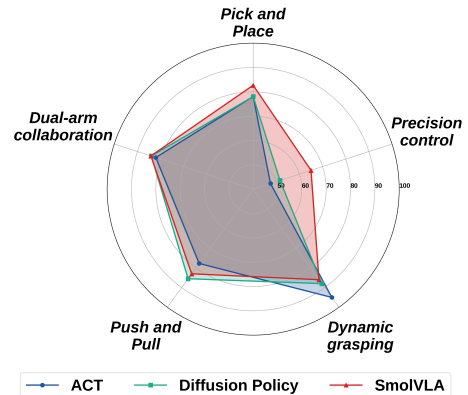
Fig. 3: Model performance comparison across different robotic skills.
