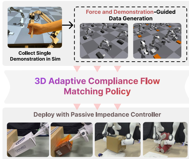
Fig. 1. Given a single demonstration in simulation, we generate force and demonstration-guided data and transfer to real-world compliant visuomotor policy deployment.
