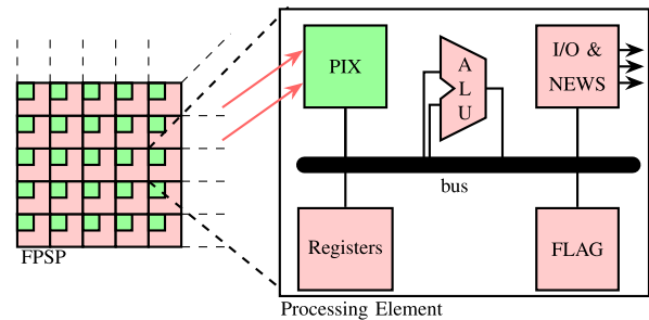
Fig. 1. In a focal-plane sensor-processor array, each pixel, i.e., processing element, combines a photosensor circuit (PIX) with on-pixel compute resources, including an arithmetic-logic unit (ALU), input/output (I/O) circuits, local communication links (NEWS), local memory (Registers), and activity control (FLAG). This architecture enables image processing to be performed directly on the sensor [5].
