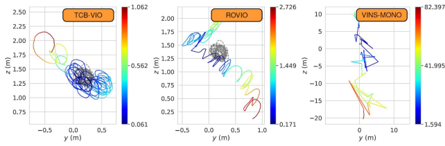
Fig. 6. Error mapping for trajectory #10, comparing TCB-VIO (left), ROVIO (middle), and VINS-Mono (right). TCB-VIO maintains low error, relative to ROVIO and VINS-MONO, closely following the ground-truth path (in gray) with minimal deviations. ROVIO shows significant drift, while VINS-Mono diverges. Note that the colorbar scales differ across the graphs.
