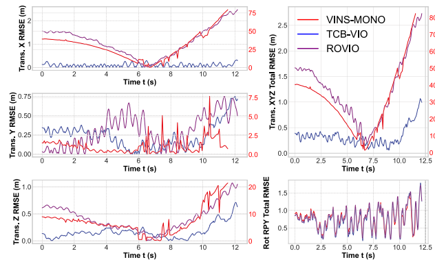
Fig. 5. Estimated RMSE for trajectory #10: (left) translation for X, Y, and Z axes, (top right) total translation, and (bottom right) total rotation. VINS-Mono has its own axes, in red, due to large error ranges. While rotational RMSE values for all three methods are close, TCB-VIO maintains the lowest overall translational RMSE.
