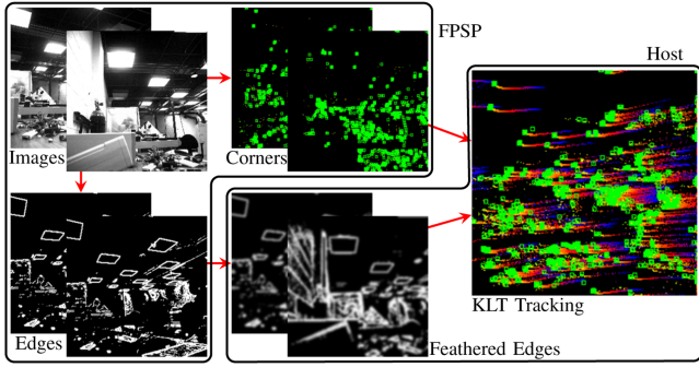
Fig. 3. Overview of the binary-enhanced KLT Tracking. The FPSP generates binary corners and edges. On the host, binary edges are feathered, and the KLT tracker operates in spatial windows centered on each corner feature.
