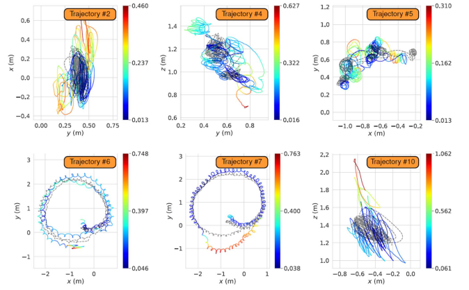
Fig. 4. Overview of representative testing trajectories used in our evaluation, aligned with the performance metrics reported in Table II. All trajectories were executed under fast and hostile motions, as reflected by the high angular velocities (10–33 rad/s) reported in Table II. Ground truth is shown in gray, with error mapping done for TCB-VIO.
