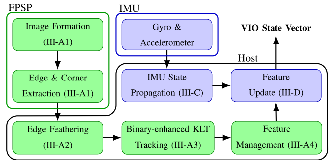
Fig. 2. TCB-VIO processing pipeline. Numbers inside each block correspond to the paper sections describing them. Green blocks denote visual processing: the FPSP performs on-sensor corner and edge extraction once an image is formed, and the extracted features are transferred to the host where a novel binary-enhanced KLT tracker ensures fast and robust tracking. Blue blocks denote inertial propagation and updates via MSCKF.
