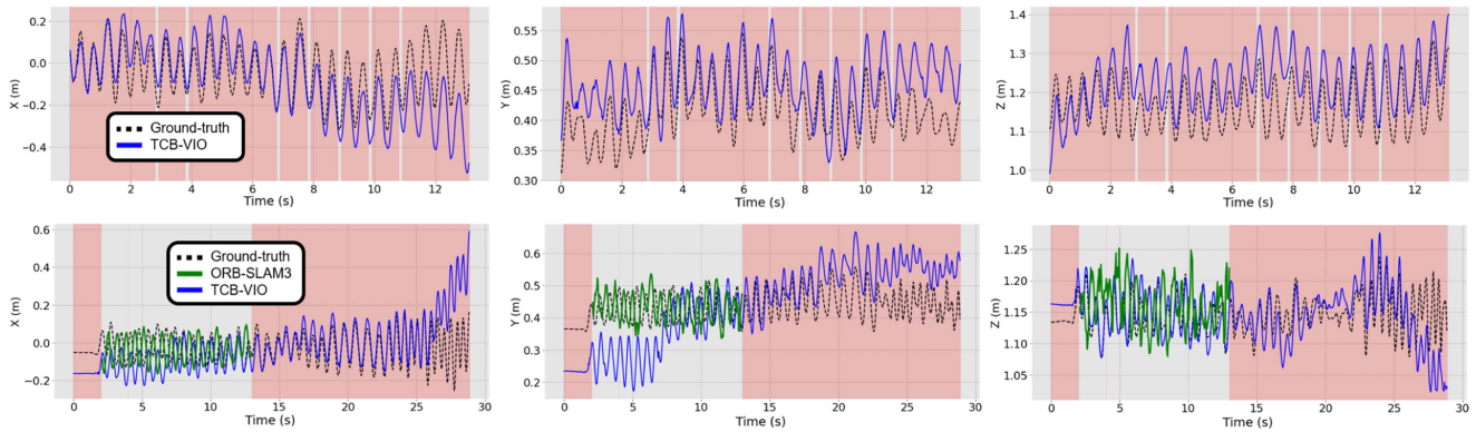
Fig. 7. (Top row) Trajectory #8 (F-type failure) showing failure during pink regions. TCB-VIO tracks consistently despite occasional deviations from ground-truth. (Bottom row) Trajectory #3 (PF-type failure) illustrating ORB-SLAM3 reinitializing but quickly diverging, highlighted in pink, leading to ATE and RTE errors.
