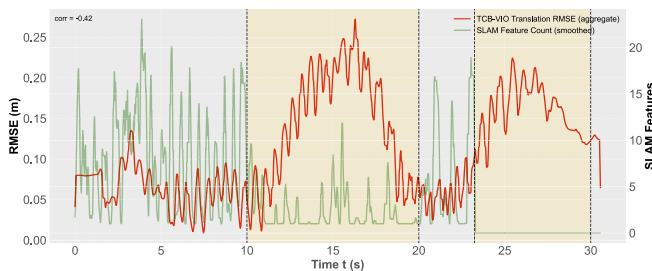
Fig. 8. Correlation between in-state feature and translational RMSE for trajectory #2. When feature count is <10 (yellow regions), TCB-VIO has higher translational RMSE.
