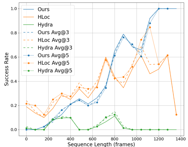
Fig. 12. Loop closure success rate over the sequence length. Avg@ X refers to the robust pose averaging in X consecutive loop frames.
