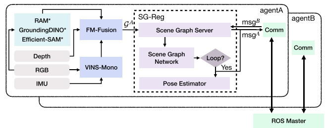
Fig. 5. Two-agent SLAM system structure. Module marked with * runs in offline.
