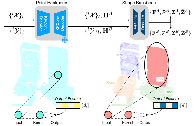
Fig. 4. Visualization of the shape network structure and its point aggregation kernels. Point backbone uses grid subsampling to decide aggregation kernels, which are small and dense. Shape backbone following instance segmentation to create aggregation kernels, which are large and sparse.
