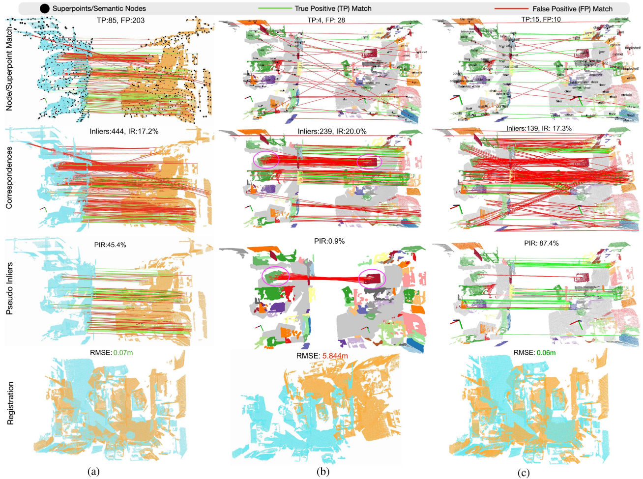
Fig. 6. Registration results in a 3RScan median scene. In SG-PGM results, the adversarial outliers are highlighted in purple circles. We annotate the corresponding evaluation metrics in each subfigure. The RMSE from a successful registration is highlighted in green, while the RMSE from a failed pair is in red. (a) GeoTransformer. (b) SG-PGM. (c) SG-Reg (Ours).
