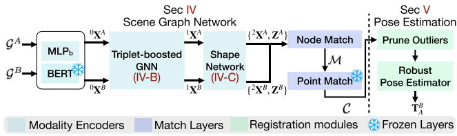
Fig. 2. Our system overview. We denote the encoded node features as {}^l\mathbf{X}^{A/B} , where its layer index l \in \{0, 1, 2\} .
