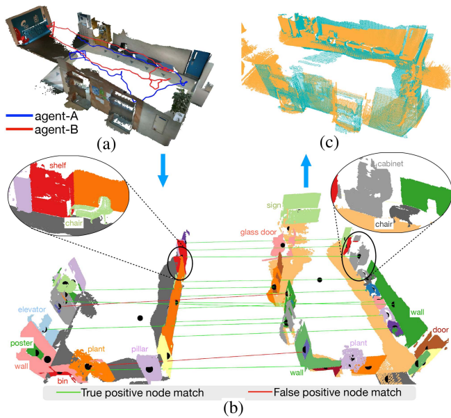
Fig. 1. Register the semantic scene graphs in the two-agent SLAM system. (a) Captured RGB-D sequences from the two agents in a real-world indoor scene. The two agents move in an opposite direction, creating a large viewpoint difference between their cameras. (b) Visualization of the matched nodes between the semantic scene graphs, which are from the two agents. The scene graphs are constructed using FM-Fusion [11]. The zoomed subvolume showcases examples of inconsistent semantic nodes. For better visualization, only a subset of the semantic labels is displayed. (c) Registration result.
