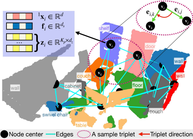
Fig. 3. Visualization of a semantic scene graph from ScanNet scene0025_00 . Each node's point cloud is distinctly colored. For node \mathbf{v}_i , we illustrate one of its triplet. In addition, the implicit features derived from \mathbf{v}_i are displayed.
