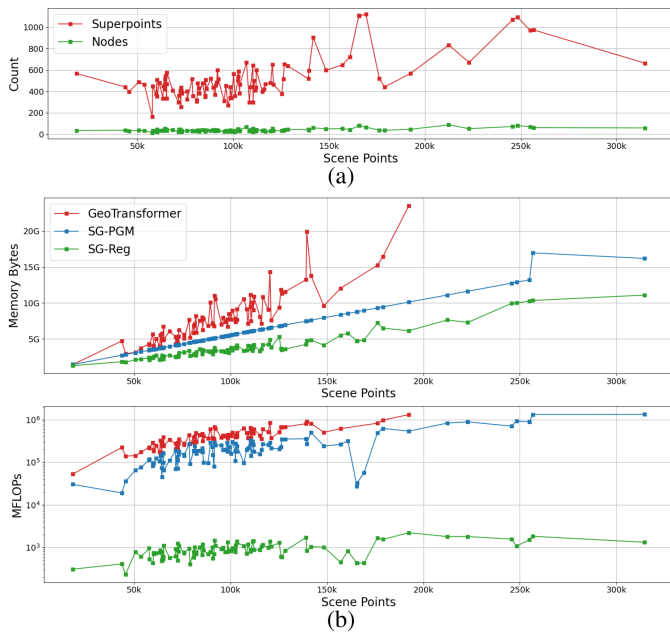
Fig. 7. (a) Sparsed 3-D representations from the 3RScan scenes in the cross-domain benchmark. (b) Reserved memory and computational complexity on a Nvidia RTX-3090 GPU. The MFLOPS are shown in exponential scales.
