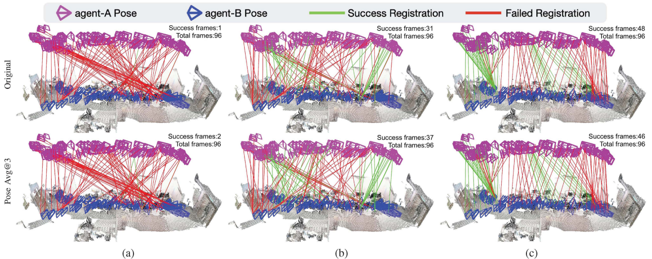
Fig. 11. Registration visualization in an office scenario. The first row shows the original results, while the second row shows the results after pose averaging using three nearest measurements. Each registration result is represented in a line. A registration is successful if its predicted camera pose has an RTE < 0.2 m and RRE < 5^\circ . For a better visualization, we align the camera poses with ground-truth transformation and incorporate a vertical translation. (a) Hydra. (b) HLoc. (c) SG-Reg (Ours).
