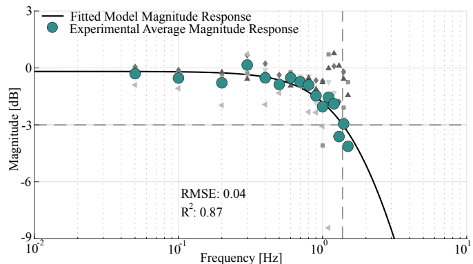
Fig. 5. Bode plot of the estimated transfer function between the measured and desired elbow position. The human-exosuit system demonstrates a bandwidth of 1.37 Hz, highlighted by the dashed line. Grey markers represent individual subject data, while green circles indicate the averaged experimental magnitude data across all participants.
