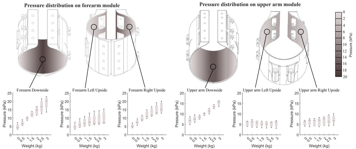
Fig. 6. Pressure distribution characterization at the human-suit interface: Measured pressures at the upper-arm and forearm cuffs under varying assistance levels under a 90 ° elbow bend. “Upside” and “Downside” in the figure refer to the upper and lower regions of each cuff, respectively.
