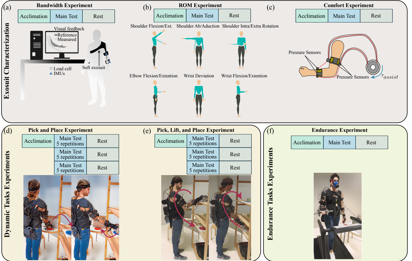
Fig. 4. Overview of the experimental procedure. (a) Protocol and schematic for the Human-in-the-loop closed-loop control bandwidth experiment. (b) Protocol and schematic for the Range of Motion and transparency experiment. (c) Protocol and schematic for the Exosuit Comfort experiment. (d, e) Protocols and schematics for the Pick and Place (P & P) and Pick, Lift, and Place (P, L & P) tasks within the dynamic session. (f) Protocol and schematic for the Endurance session experiment.
