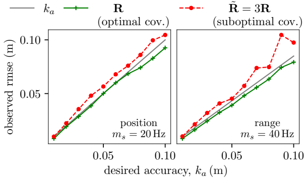
Fig. 4. Trajectory estimation results from simulation using position sensors (left) and range sensors (right) of proposed covariance, \mathbf{R} (optimal cov.), and higher covariance, \tilde{\mathbf{R}} = 3\mathbf{R} (suboptimal cov.). The desired RMSE for a given accuracy value, k_a , is indicated by the black line in each case. Using sensors with the proposed covariances, the trajectory estimation RMSE is lower than the desired accuracy k_a in each case. However, using sensors with higher covariances results in RMSE higher than the required accuracy, indicating the validity of our approach.
