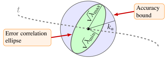
Fig. 2. The error correlation matrix, \check{\mathbf{P}}_{\mathbf{x}_t} , viewed as the ellipse \{\mathbf{x} \in \mathbb{R}^2 \mid \mathbf{x}^T (\check{\mathbf{P}}_{\mathbf{x}_t})^{-1} \mathbf{x} \leq 1\} (green), represents the spread of errors and the square root of its maximum eigenvalue, \sqrt{\lambda_{\max}} , gives the maximum error along any principle axis. To achieve desired accuracy k_a , the error ellipse must be within the accuracy bound ellipse \{\mathbf{x} \in \mathbb{R}^2 \mid \mathbf{x}^T (k_a^2 \mathbf{I})^{-1} \mathbf{x} \leq 1\} (blue) at each time step t (gray dashed line).
